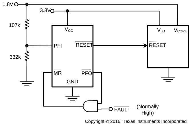
Figure 15. Monitoring Dual Supplies Plus External Fault Input
