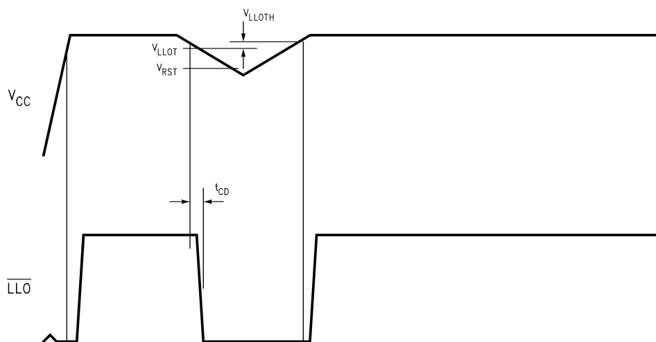
Figure 2. \overline{LLO} Output
