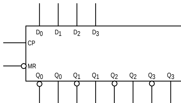
LOGIC SYMBOL
