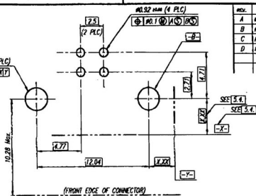
FIGURE A: PCB FOOTPRINT FOR RECEPTACLE (THROUGH-HOLE)
