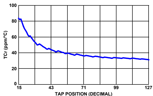
FIGURE 16. 50kΩ TCcr vs TAP POSITION, V_{CC} = 3.3V
