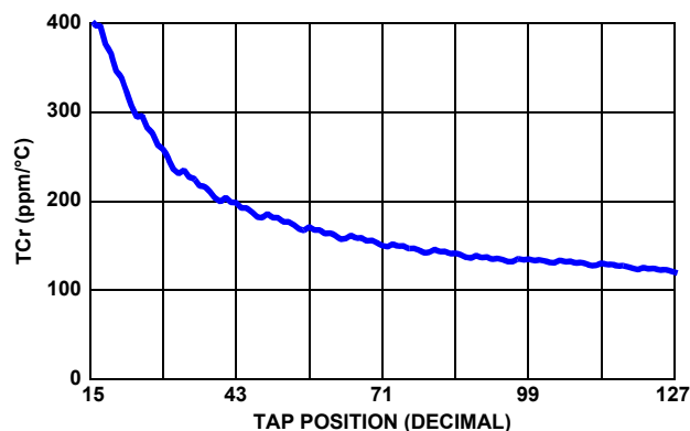
FIGURE 15. 10kΩ TCcr vs TAP POSITION
