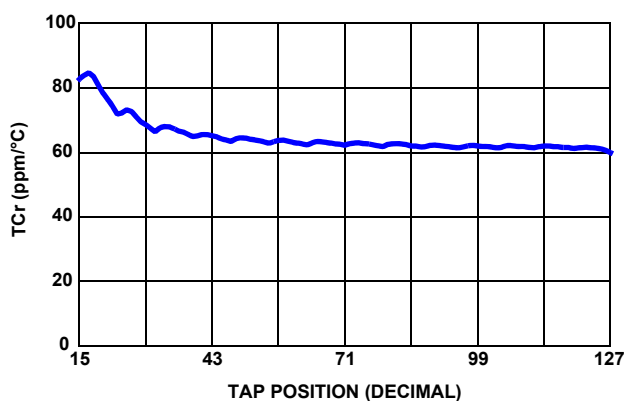
FIGURE 18. 100kΩ TCcr vs TAP POSITION, V_{CC} = 3.3V
