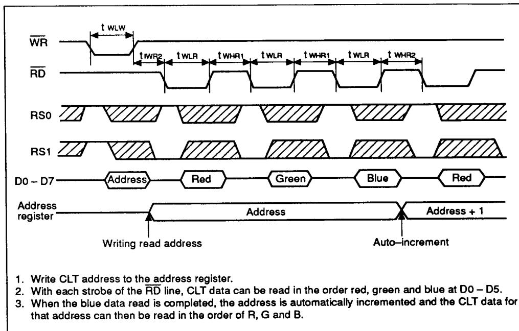
Figure 8 CLT Read
