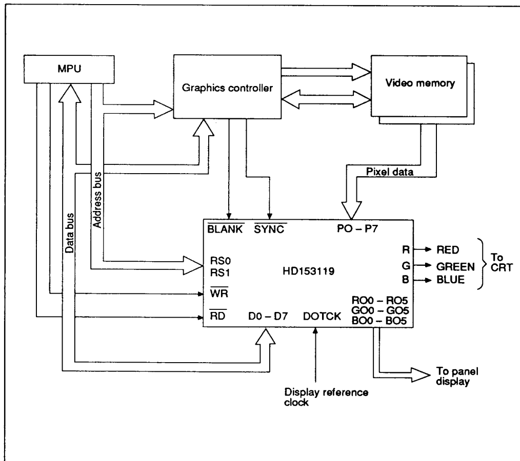
Figure 18 System Configuration Example
