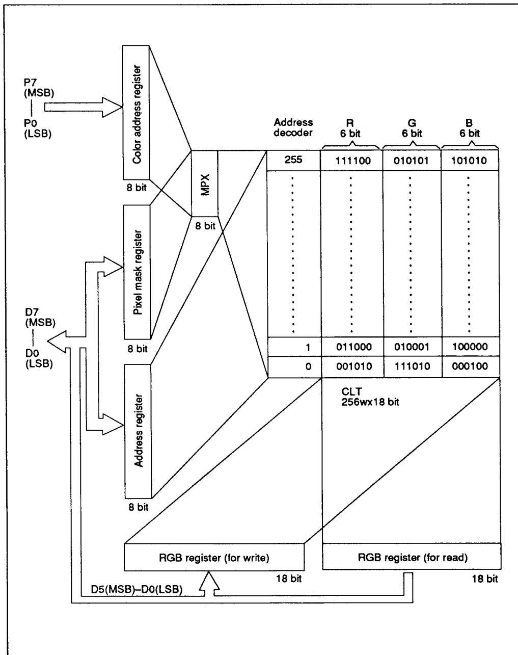
Figure 17 Register Correspondence with CLT
