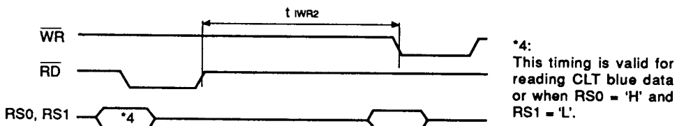
Figure 6 Write after Read
