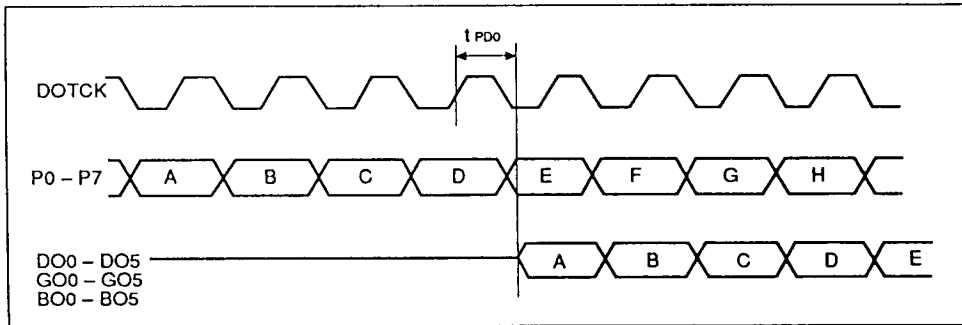
Figure 12 Digital Output
