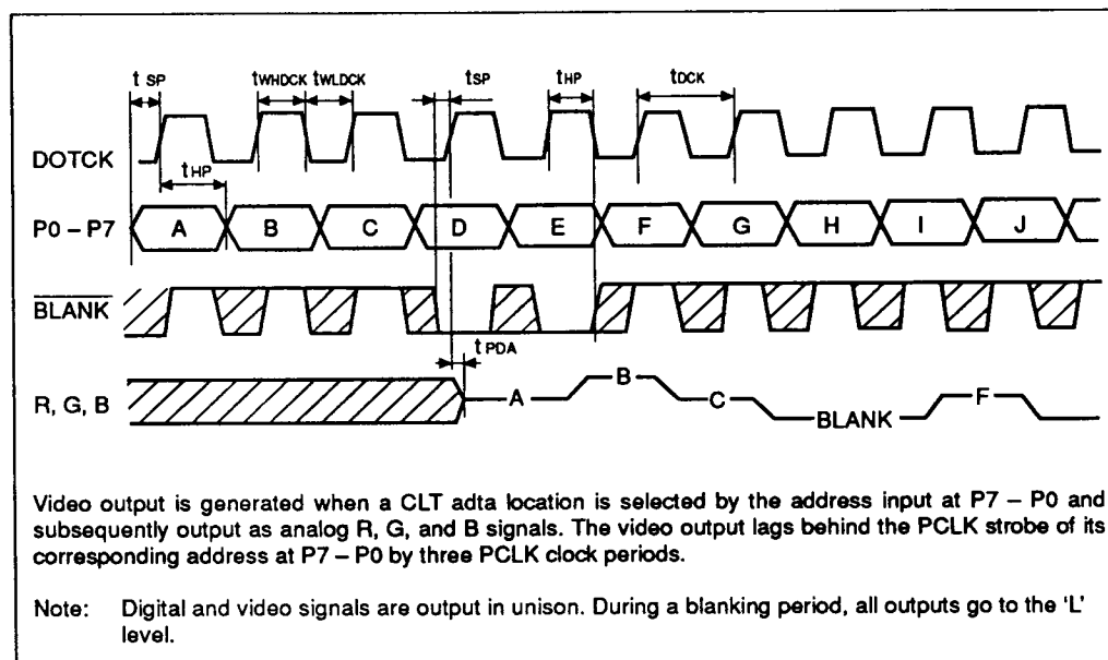
Figure 9 Video Output
