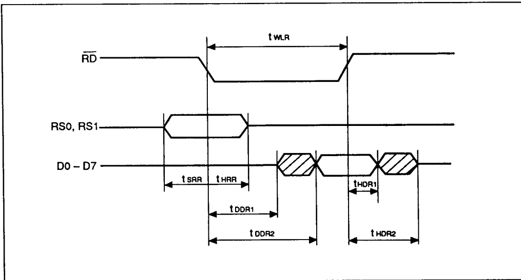
Figure 4 Read Timing
