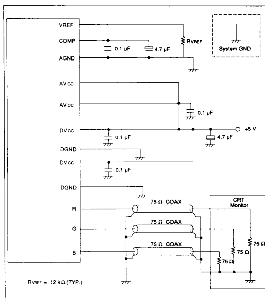
Figure 19 Connection Example
