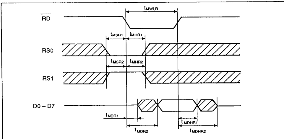
Figure 14 Pixel Mask Register Read
