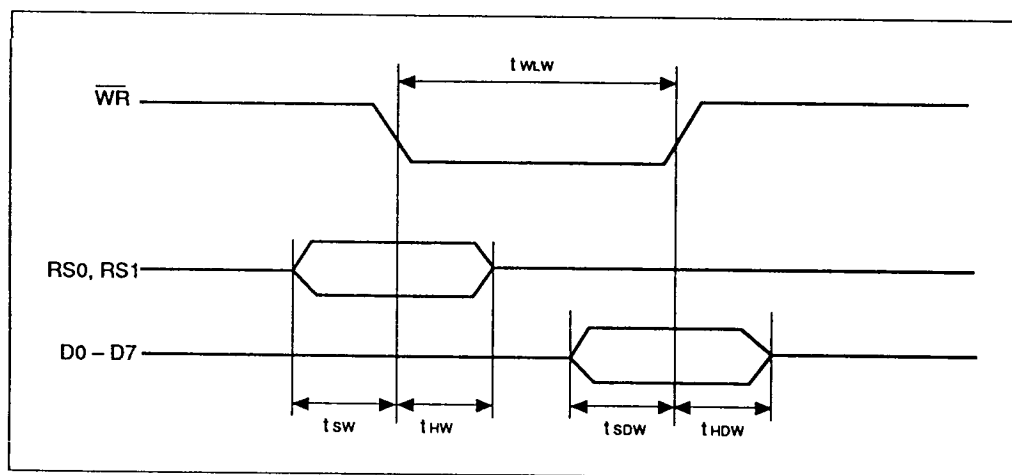
Figure 3 Write Timing
