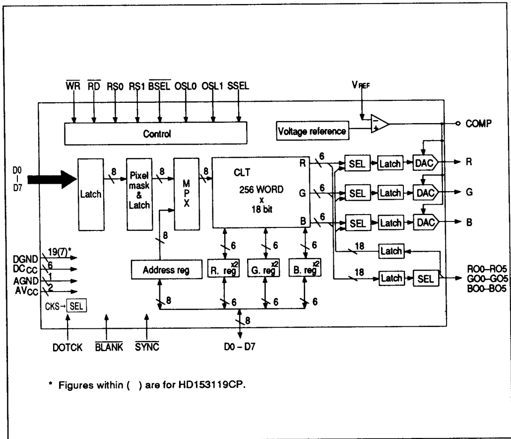
Figure 2 Block Diagram
