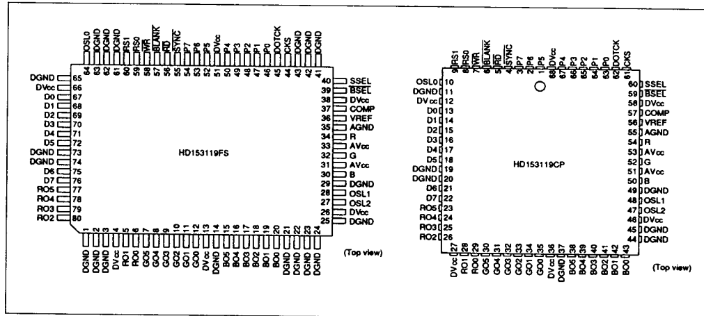
Figure 1 Pin Arrangement
