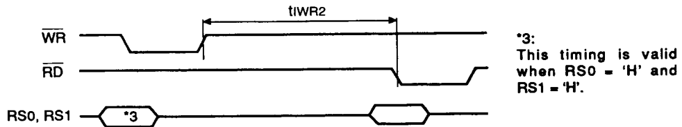
Figure 5 Read after Write
