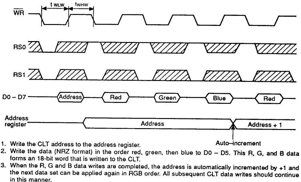
Figure 7 CLT Write
