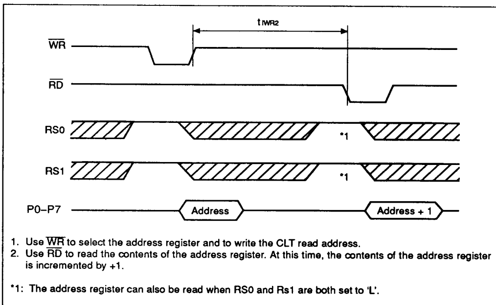
Figure 10 Address Register Read (1)
