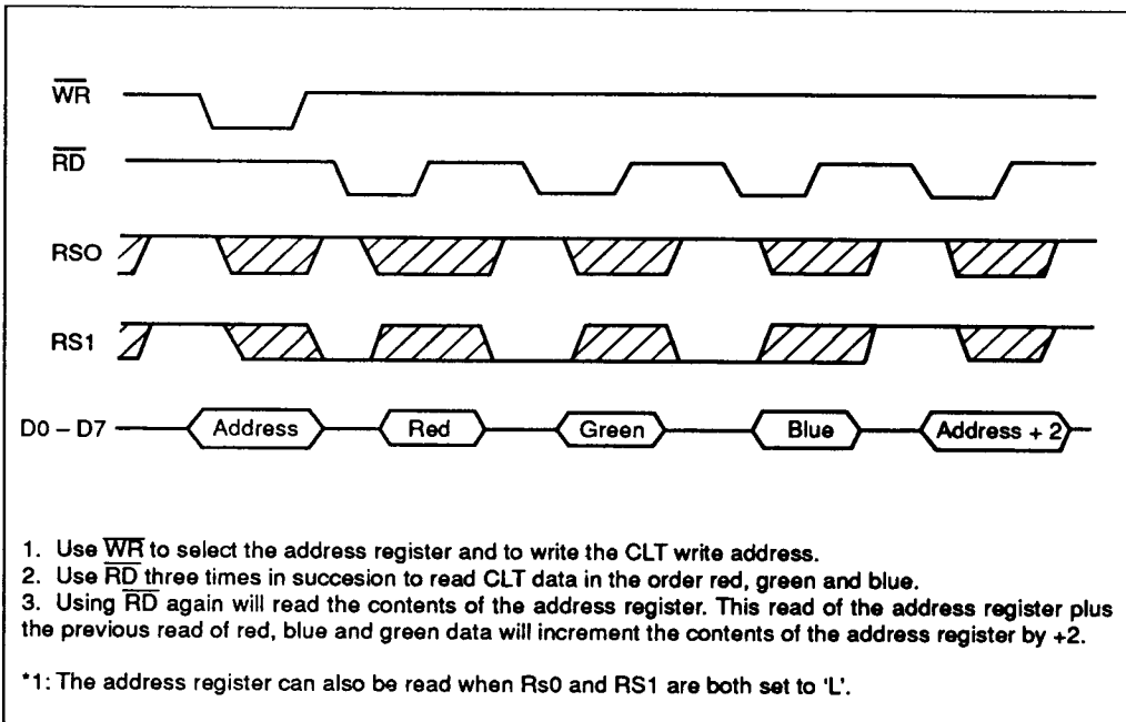
Figure 11 Address Register Read (2)
