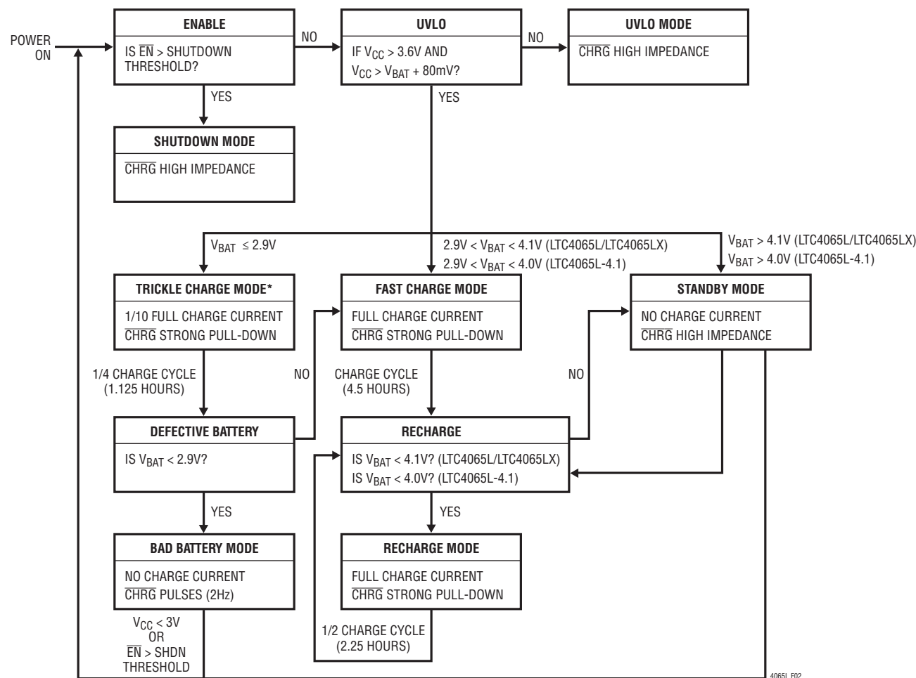
Figure 2. State Diagram of LTC4065L Operation
