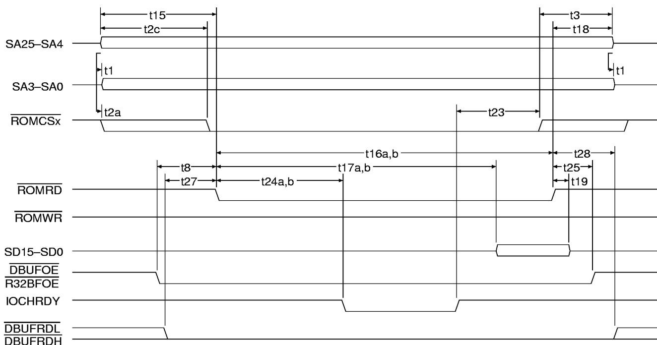
Figure 30. Normal Mode 8-/16-Bit ROM/Flash Memory Read Cycles
