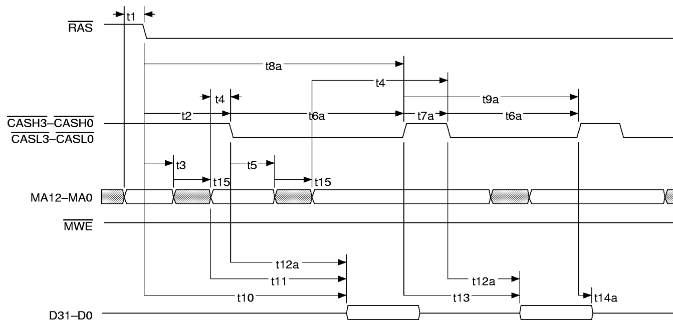
Figure 35. DRAM Page Hit Read, Non-Interleaved
