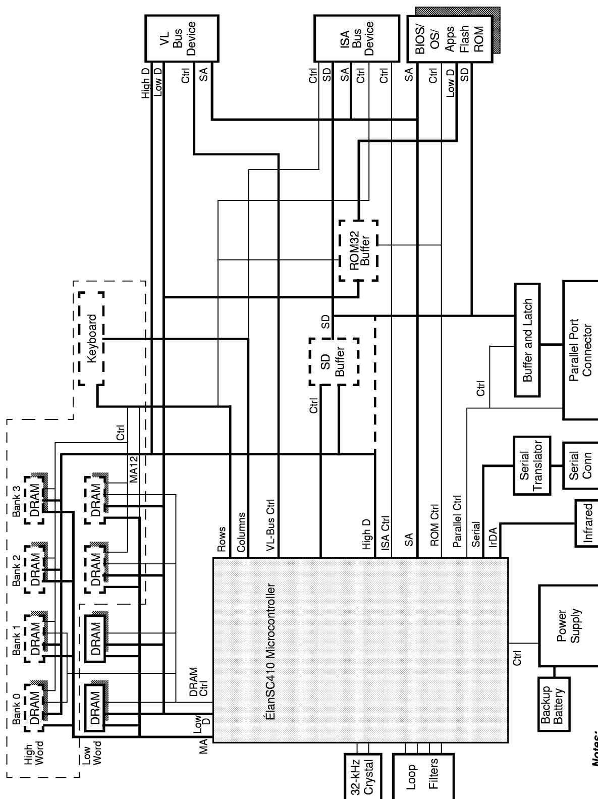
Figure 3. System Design with Trade-offs—ÉlanSC410 Microcontroller
