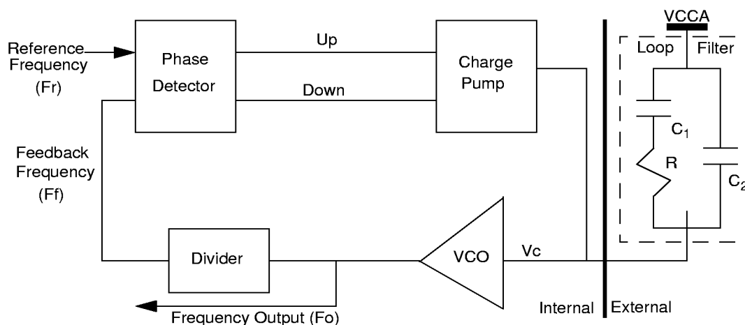
Figure 8. Intermediate and Low-Speed PLLs Block Diagram
