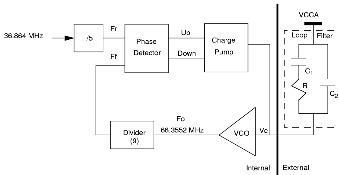
Figure 10. High-Speed PLL Block Diagram
