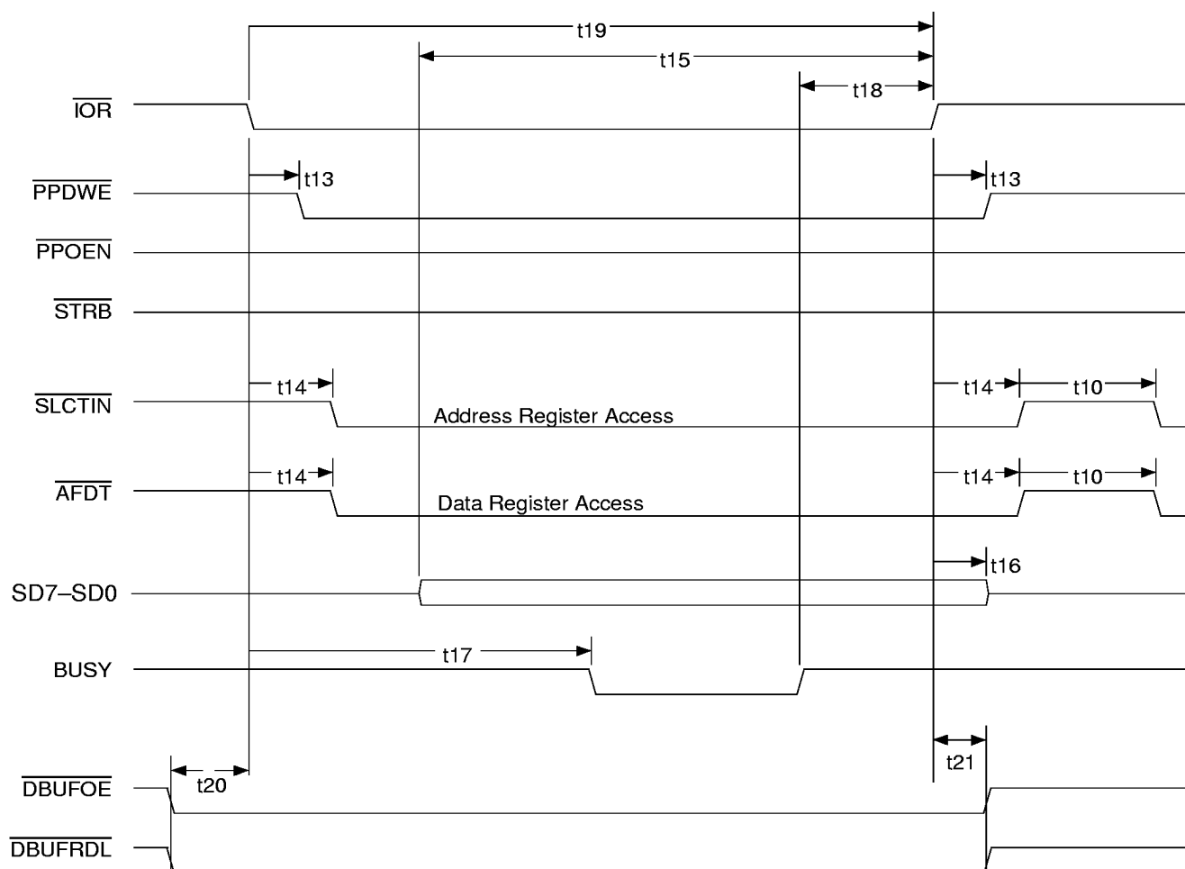
Figure 49. EPP Parallel Port Read Cycle
