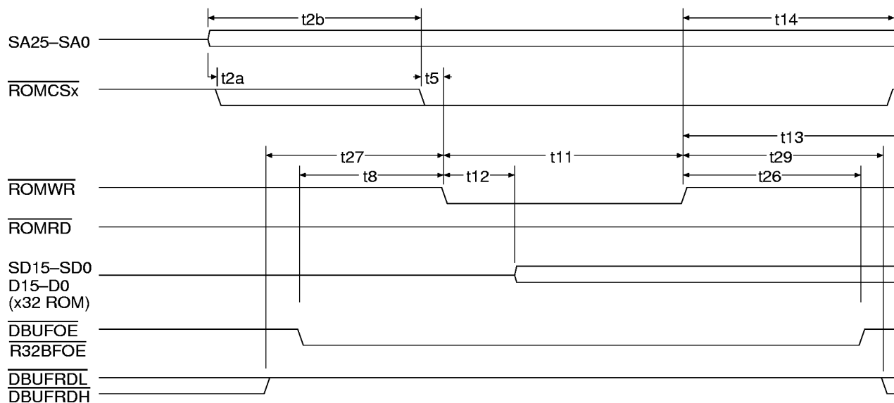
Figure 27. Fast Mode 8-/16-/32-Bit Flash Memory Write Cycles
