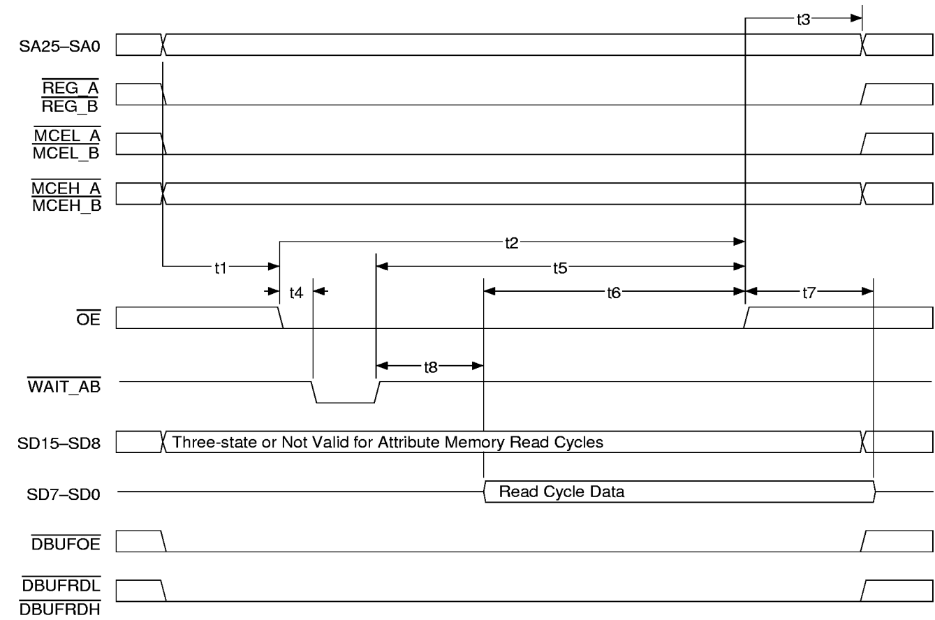
Figure 55. PC Card Attribute Memory Read Cycle (ÉlanSC400 Microcontroller Only)
