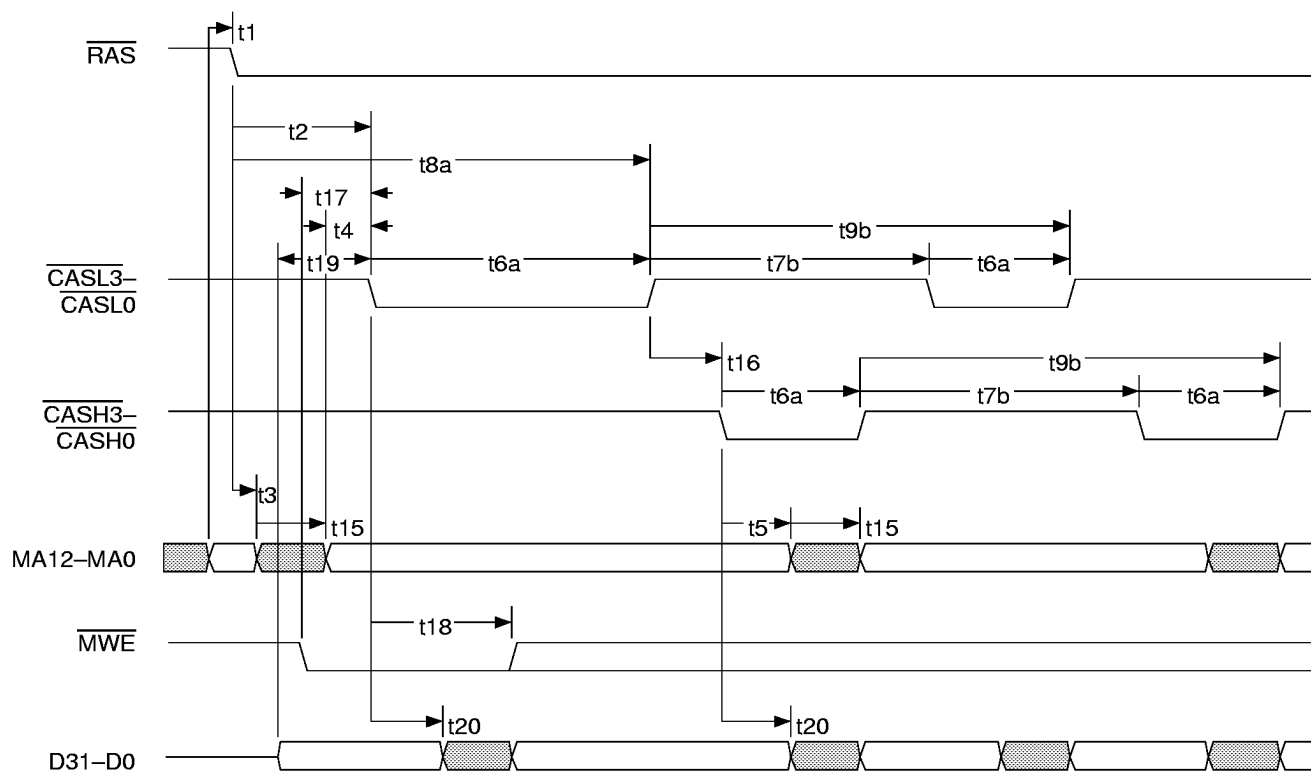
Figure 33. DRAM Page Hit Write, Interleaved
