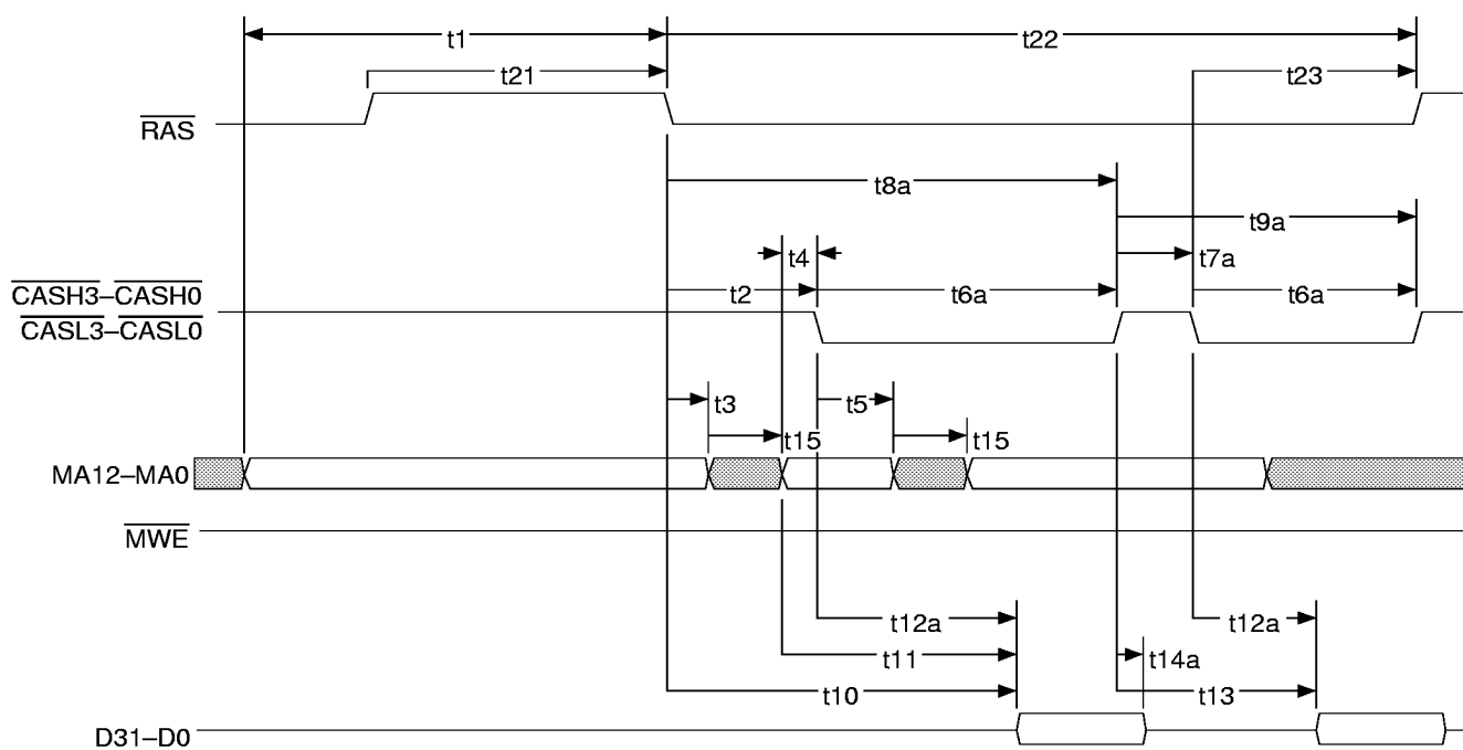
Figure 37. DRAM Page Miss Read, Non-Interleaved
