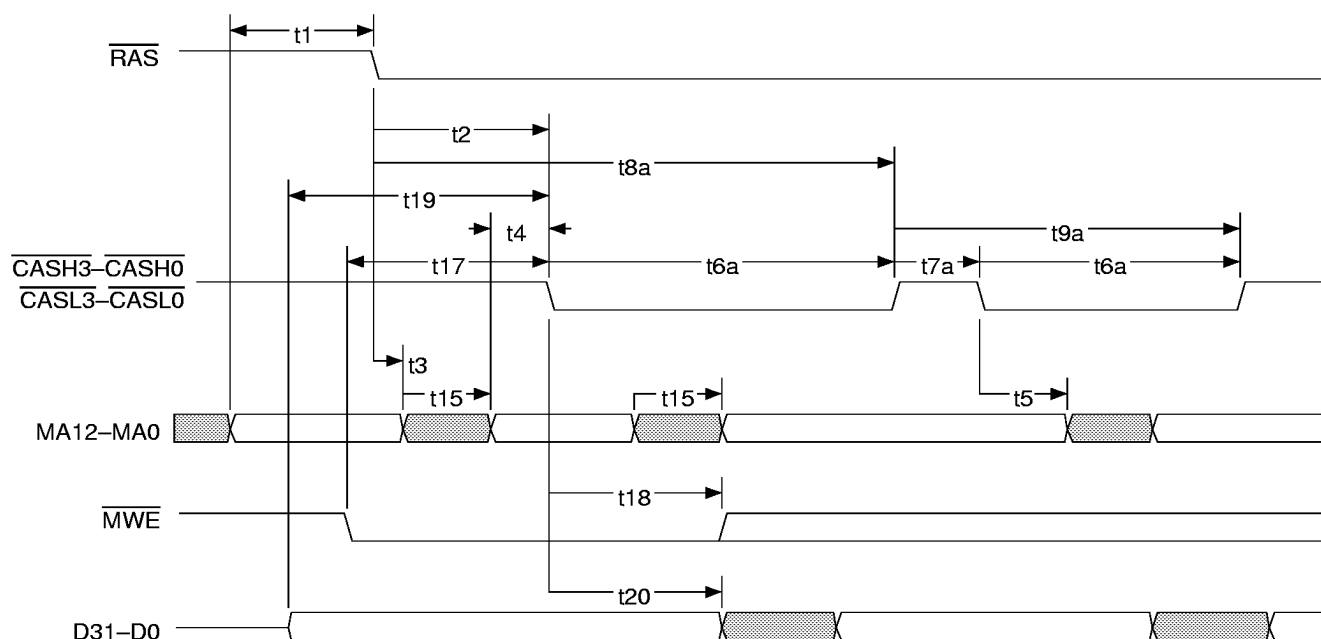
Figure 36. DRAM Page Hit Write, Non-Interleaved
