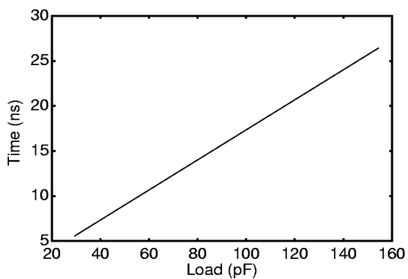
Figure 19. 3.3-V I/O Drive Type C Fall Time
