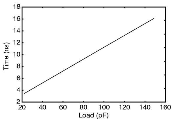
Figure 20. 3.3-V I/O Drive Type D Rise Time
