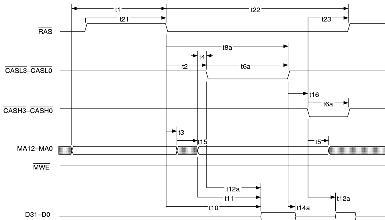
Figure 34. DRAM Page Miss Read, Interleaved
