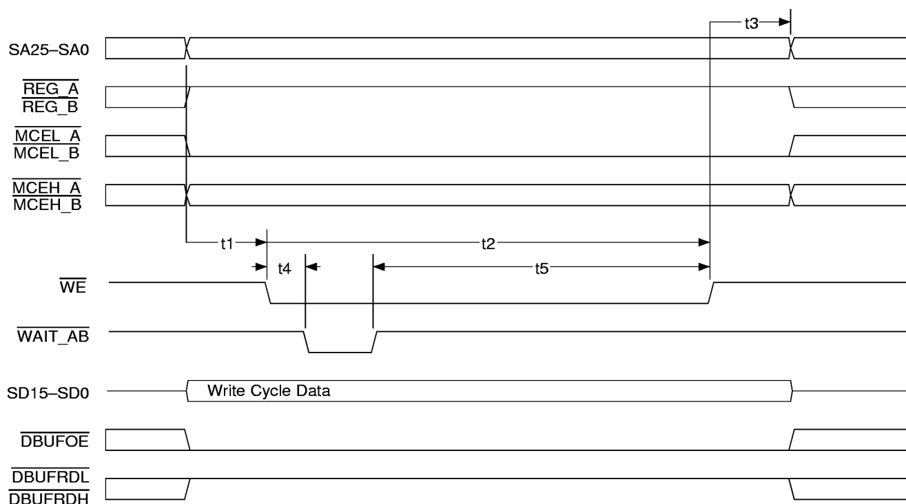
Figure 58. PC Card Common Memory Write Cycle (ÉlanSC400 Microcontroller Only)
