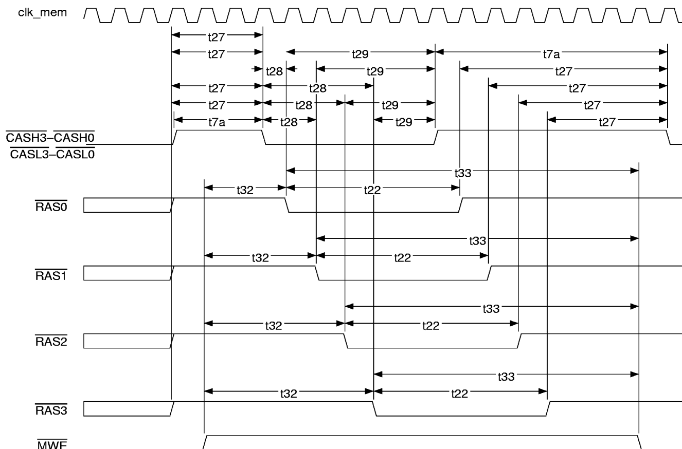
Figure 40. DRAM CAS-Before-RAS Refresh
