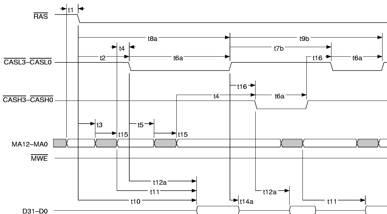
Figure 32. DRAM Page Hit Read, Interleaved
