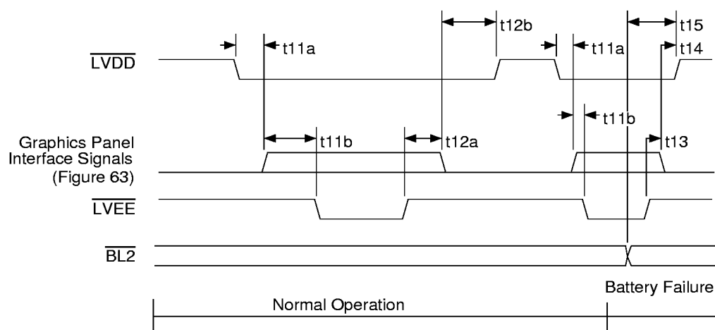
Figure 64. Graphics Panel Power Sequencing (ÉlanSC400 Microcontroller Only)
