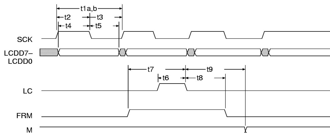
Figure 63. Graphics Panel Interface Timing (ÉlanSC400 Microcontroller Only)
