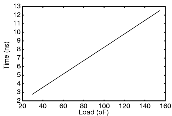
Figure 23. 3.3-V I/O Drive Type E Fall Time
