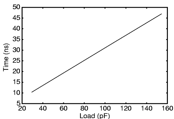
Figure 16. 3.3-V I/O Drive Type B Rise Time
