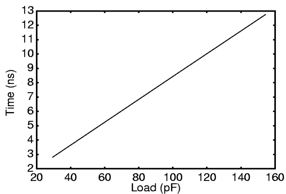
Figure 22. 3.3-V I/O Drive Type E Rise Time
