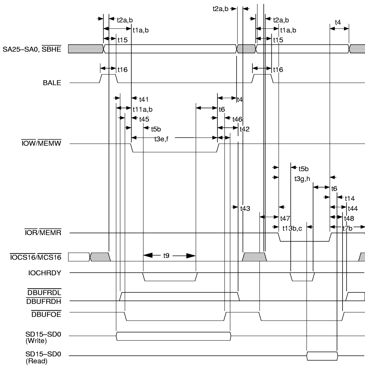
Figure 44. 16-Bit ISA Bus Cycles
