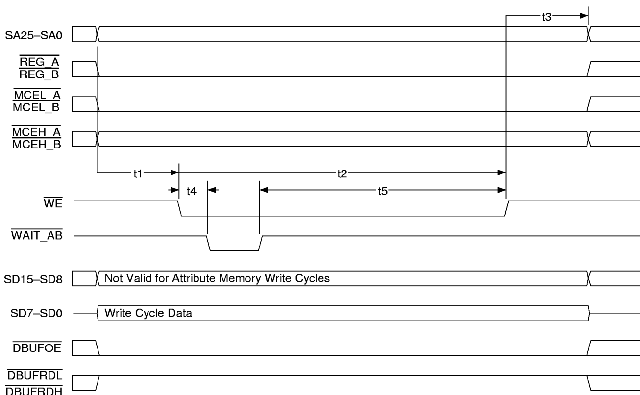
Figure 56. PC Card Attribute Memory Write Cycle (ÉlanSC400 Microcontroller Only)
