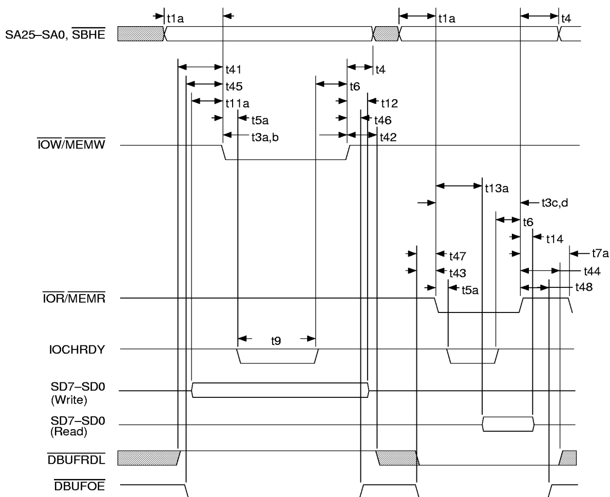
Figure 43. 8-Bit ISA Bus Cycles
