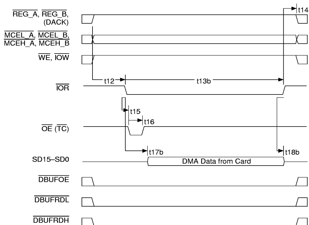
Figure 62. PC Card DMA Write Cycle (I/O Read to Memory Write)
