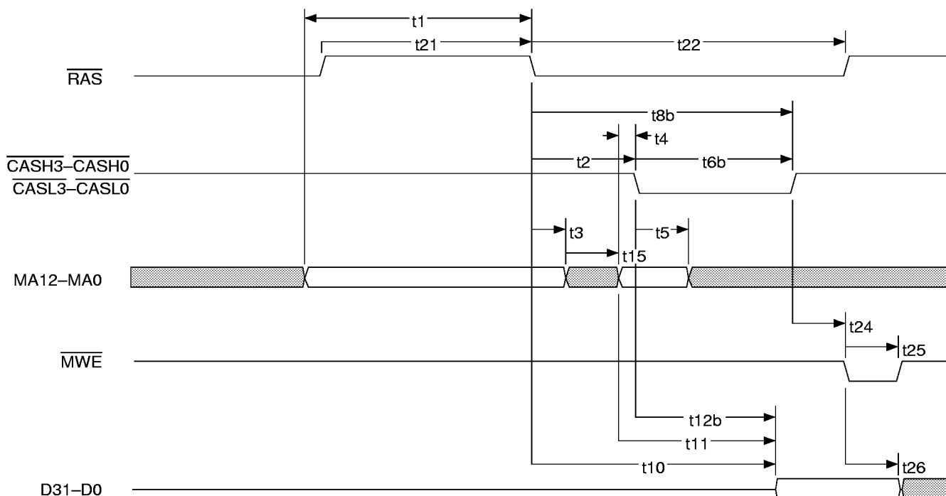
Figure 38. EDO DRAM Page Hit Read, Non-Interleaved
