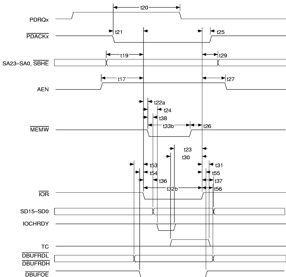
Figure 46. ISA DMA Write Cycle
