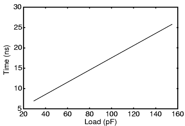
Figure 18. 3.3-V I/O Drive Type C Rise Time
