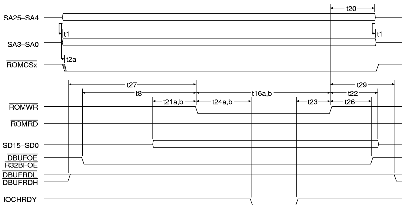
Figure 31. Normal Mode 8-/16-Bit Flash Memory Write Cycles
