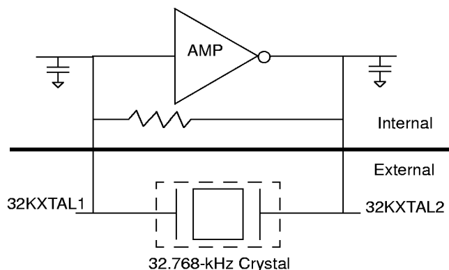
Figure 6. 32-kHz Crystal Circuit
