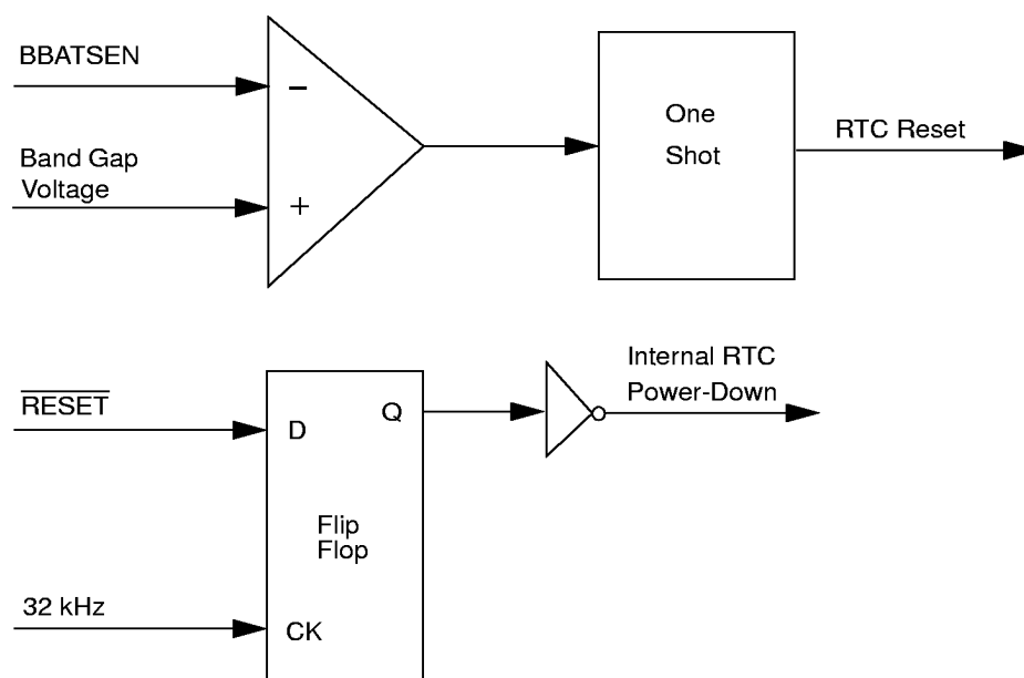
Figure 11. RTC Voltage Monitor Circuit
