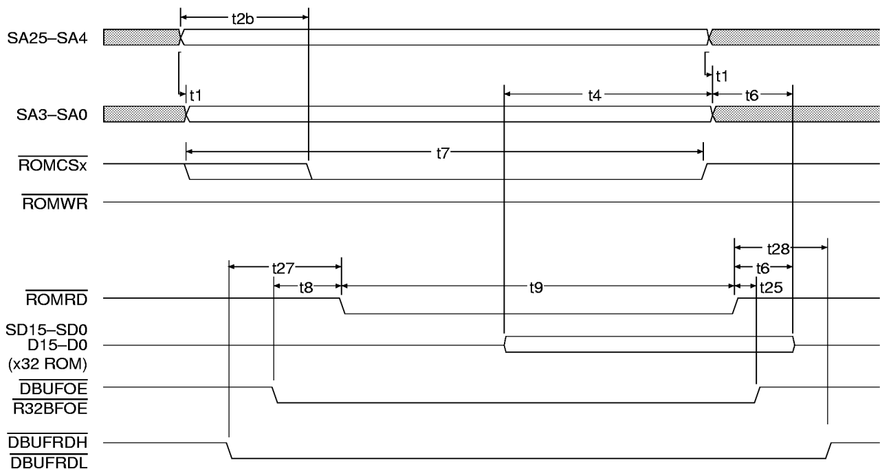
Figure 25. Fast Mode 8-/16-/32-Bit ROM/Flash Memory Read Cycle
