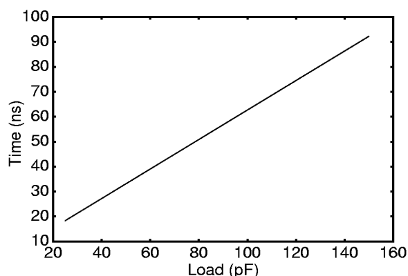
Figure 15. 3.3-V I/O Drive Type A Fall Time
