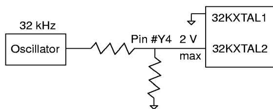
Figure 7. 32-kHz Oscillator Circuit
