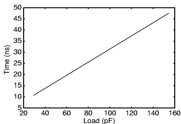
Figure 17. 3.3-V I/O Drive Type B Fall Time
