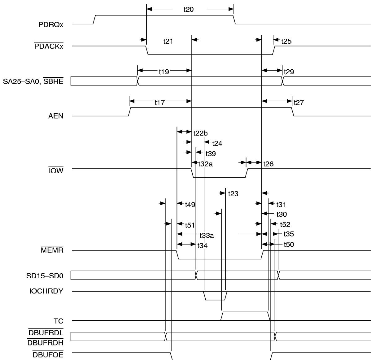
Figure 45. ISA DMA Read Cycle
