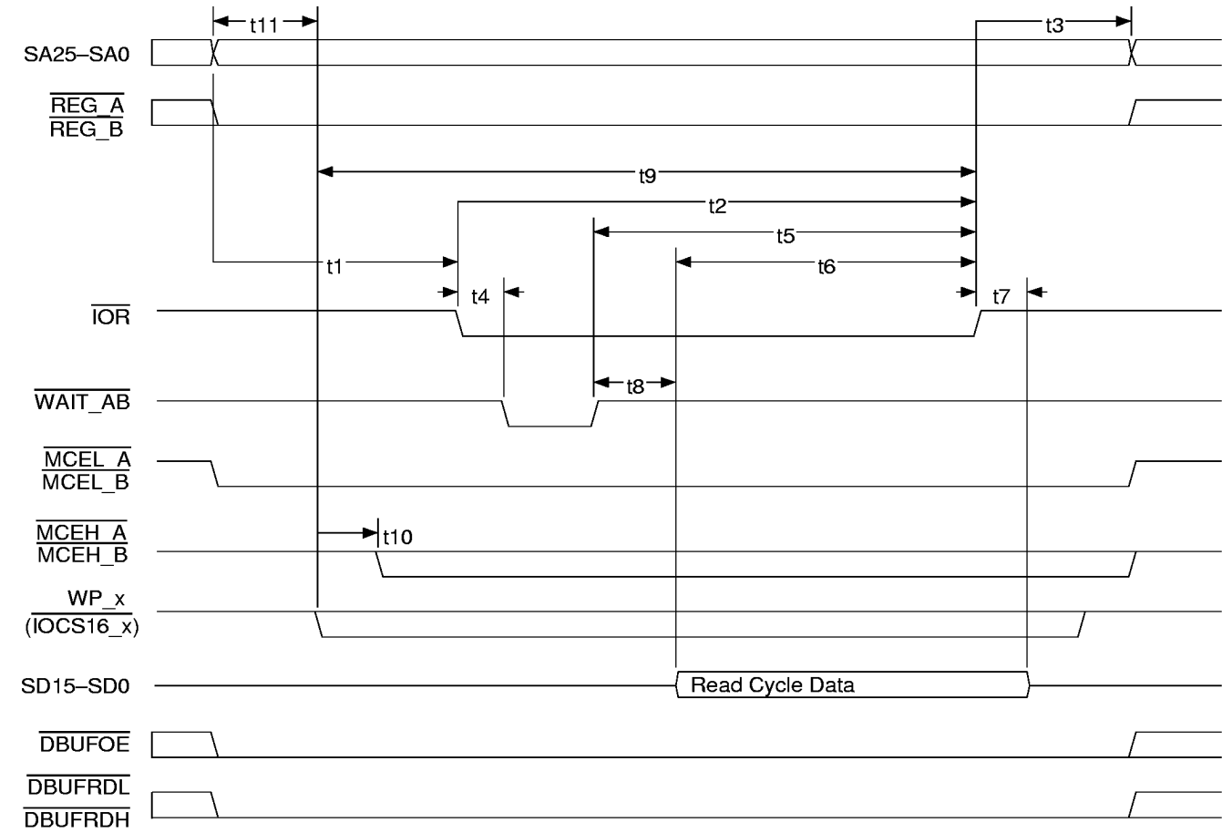
Figure 59. PC Card I/O Read Cycle
