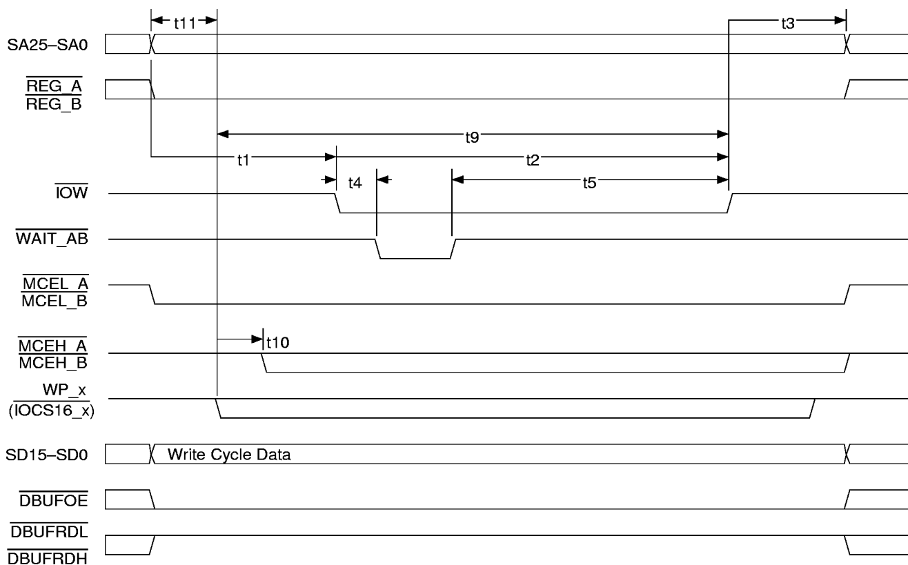
Figure 60. PC Card I/O Write Cycle
