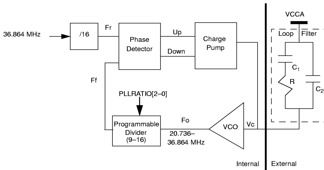
Figure 9. Graphics Dot Clock PLL Block Diagram
