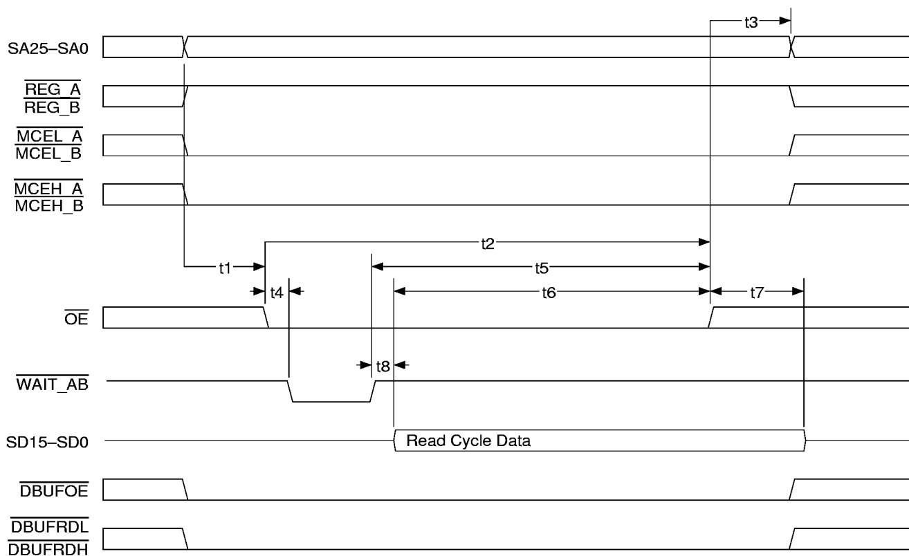
Figure 57. PC Card Common Memory Read Cycle (ÉlanSC400 Microcontroller Only)
