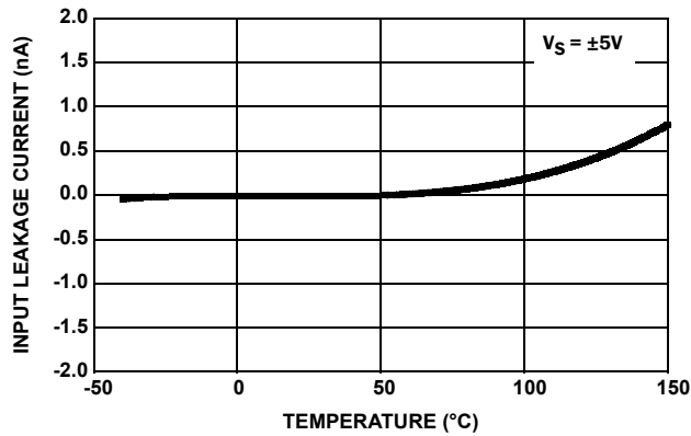
FIGURE 3. INPUT LEAKAGE CURRENT vs TEMPERATURE
