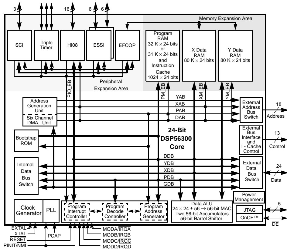
Figure 1. DSP56321 Block Diagram
