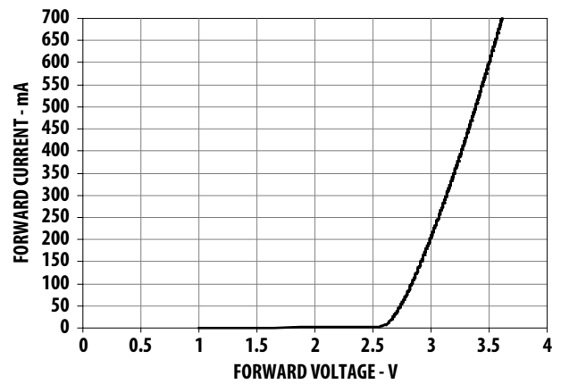
Figure 15. Forward Current vs. Forward Voltage.
