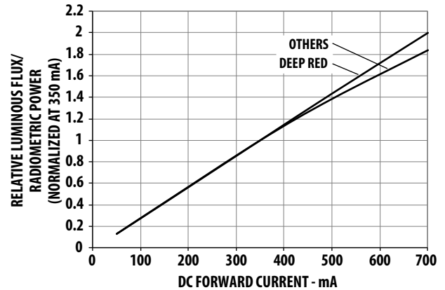
Figure 3. Relative Luminous Flux/ Radiometric Power vs. Mono Pulse Current.
