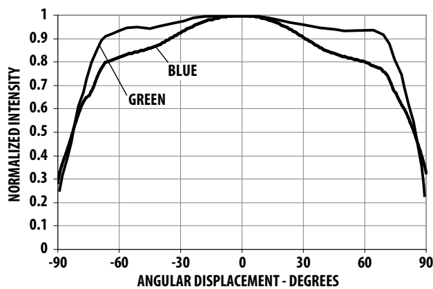
Figure 16. Radiation Pattern for Blue and Green.
