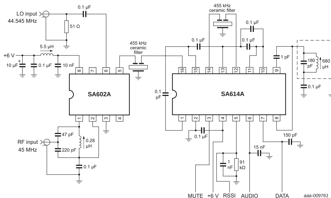
Fig 6. Typical application cellular radio (45 MHz RF input and 455 kHz IF)
