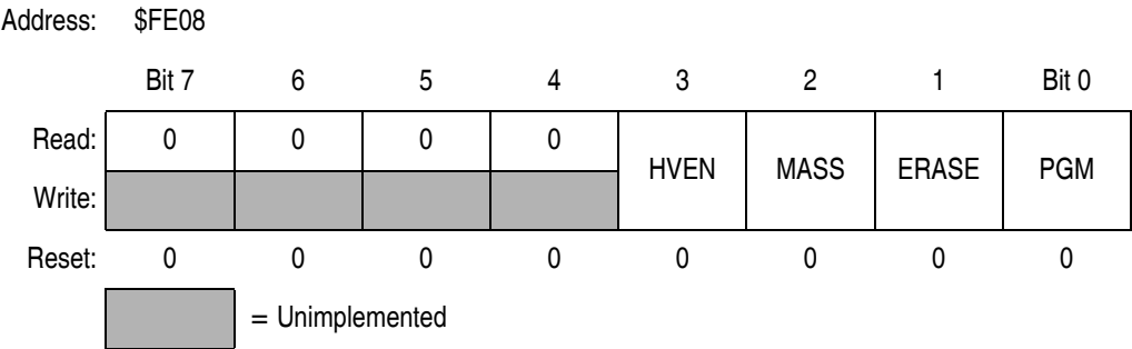
Figure 4-2. FLASH Control Register (FLCR)
