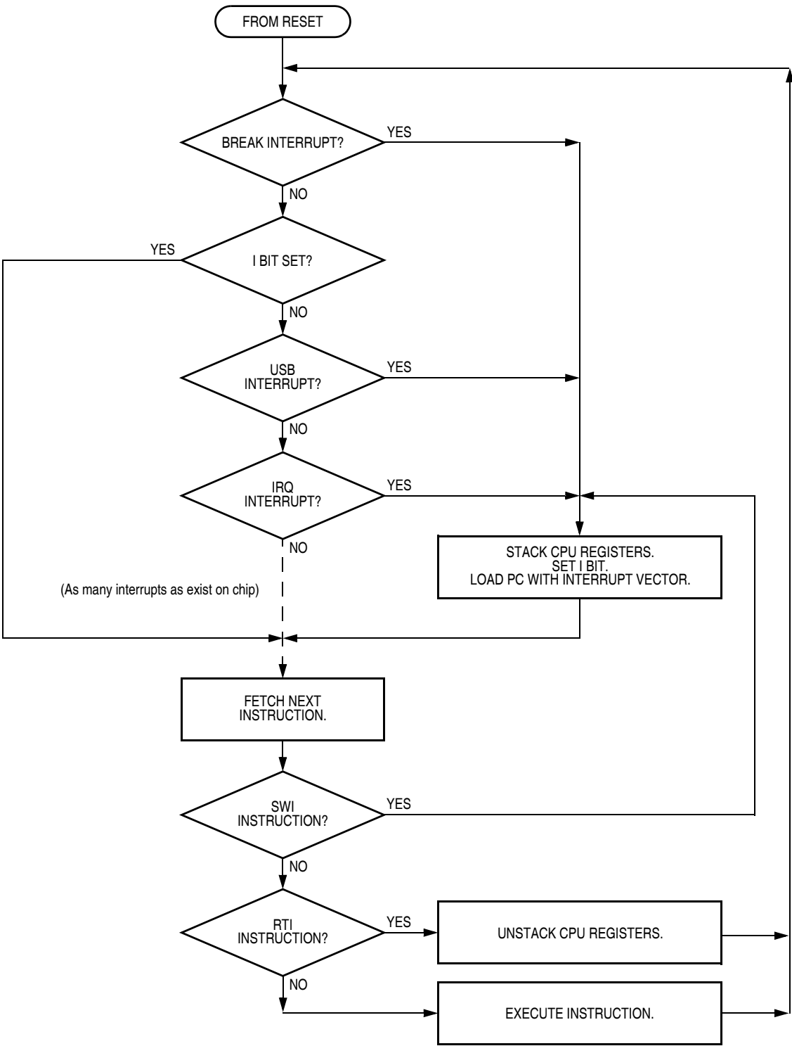
Figure 8-8. Interrupt Processing
