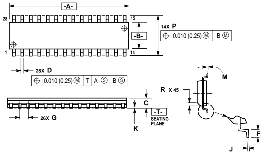
Figure 21-2. 28-Pin SOIC (Case #751F)
