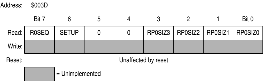
Figure 11-24. USB Status Register 0 (USR0)
