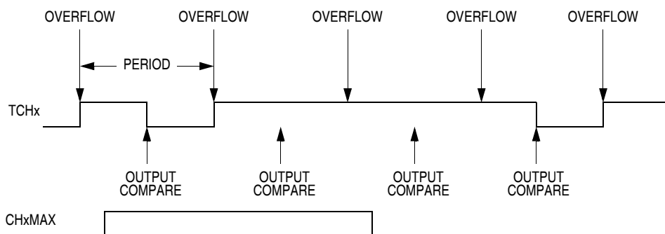
Figure 10-11. CHxMAX Latency
