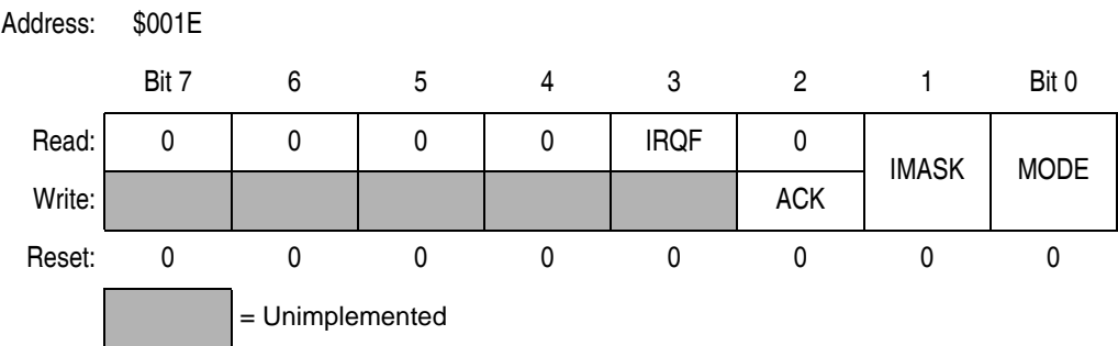
Figure 15-3. IRQ Status and Control Register (ISCR)
