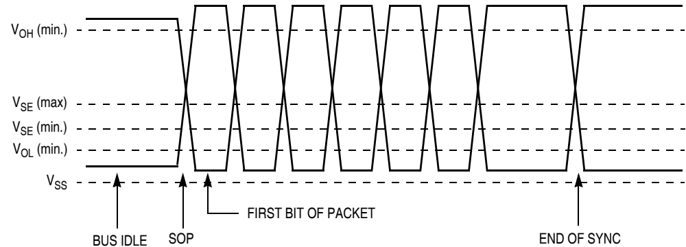
Figure 11-6. SOP, Sync Signaling, and Voltage Levels
