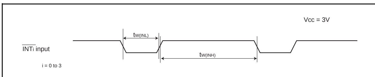
Figure 5.15 External Interrupt \overline{INTi} Input Timing Diagram when VCC = 3 V
