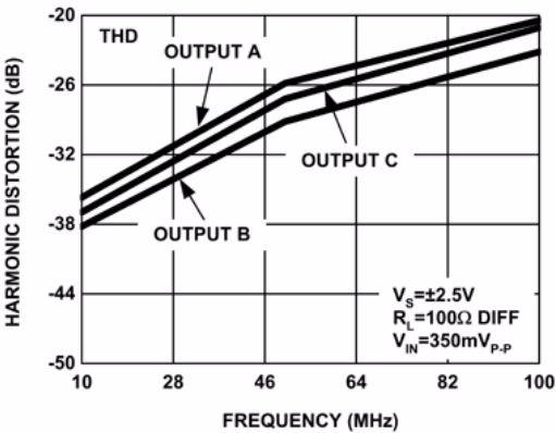
FIGURE 33. HARMONIC DISTORTION
