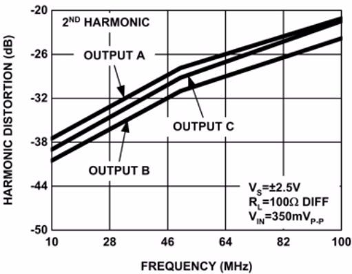
FIGURE 31. HARMONIC DISTORTION
