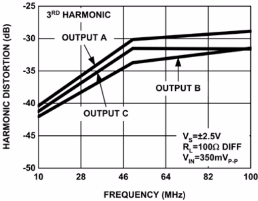
FIGURE 32. HARMONIC DISTORTION
