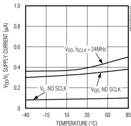
V_{DD}/V_L FULL POWER-DOWN SUPPLY CURRENT vs. TEMPERATURE
