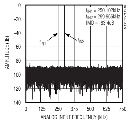
TWO-TONE IMD PLOT (MAX1071)
