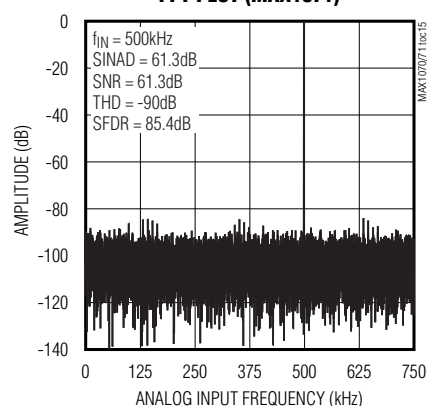
FFT PLOT (MAX1071)
