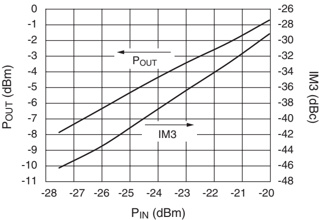
Output Power and Relative Third-Order Intermodulation Products F = 38\text{ GHz} , V_{D1} = V_{D2} = 4.5\text{ V}
