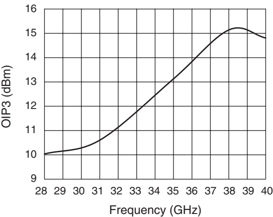
Two-Tone Output Third-Order Intercept @ V_{D1} = V_{D2} = 4.5\text{ V}
