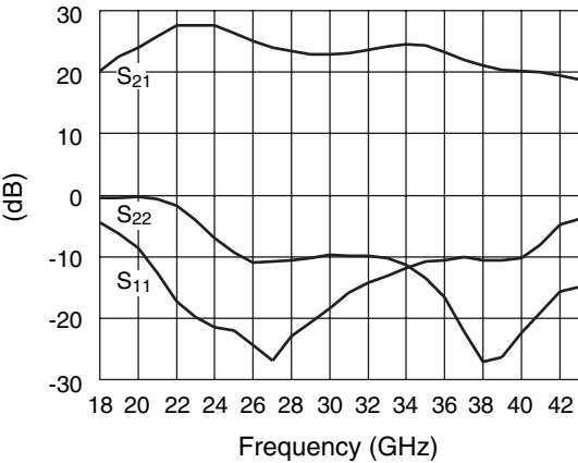
Typical Small Signal Performance S-Parameters (V D = 4.5 V)
