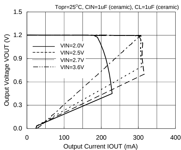
XC6209B122
