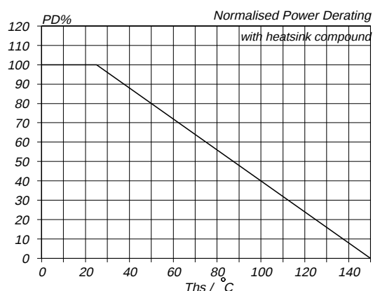
Fig.10. Normalised power dissipation. PD\% = 100 \cdot PD / PD\ 25^\circ\text{C} = f(T_{bs})
