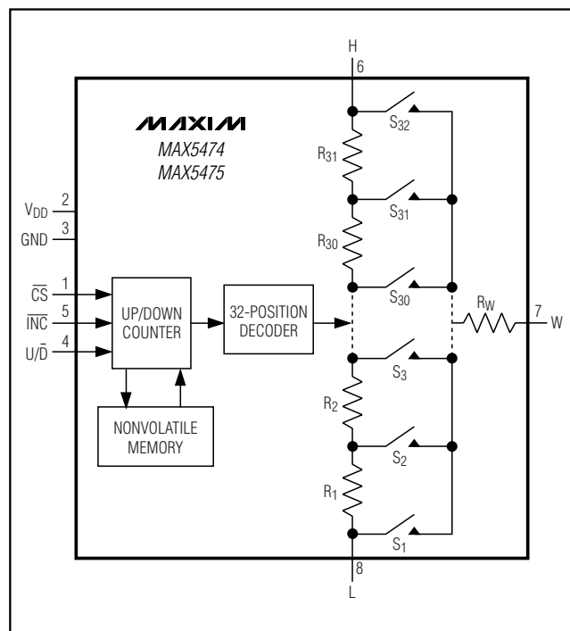
Figure 3. MAX5474/MAX5475 Functional Diagram
