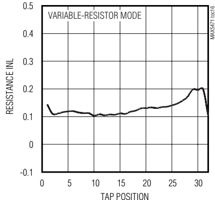
RESISTANCE INL vs. TAP POSITION (MAX5472)
