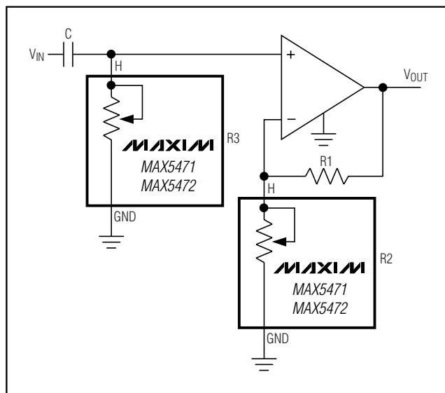
Figure 6. Programmable Filter
