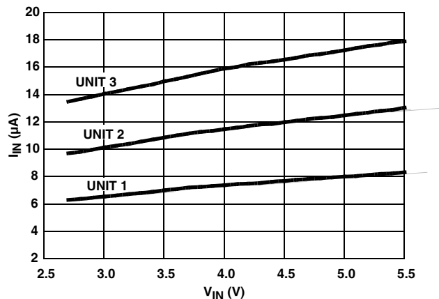
FIGURE 1. I_{IN} vs V_{IN} (3 REPRESENTATIVE UNITS)
