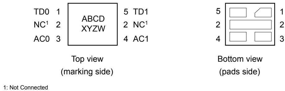
Figure 3. Die connections for sawn and bumped wafer (bottom view)
