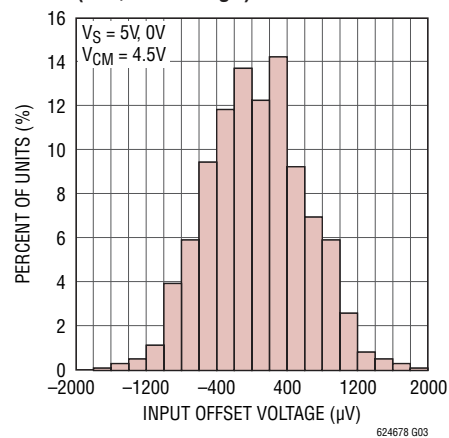
V_{OS} Distribution, V_{CM} = V^+ - 0.5V (MS, NPN Stage)
