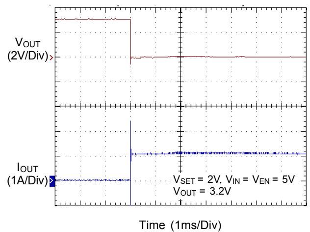
Short-Circuit Protection
