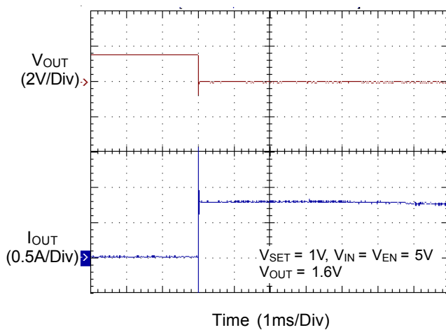
Short-Circuit Protection
