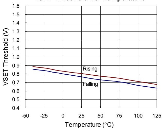
VSET Threshold vs. Temperature
