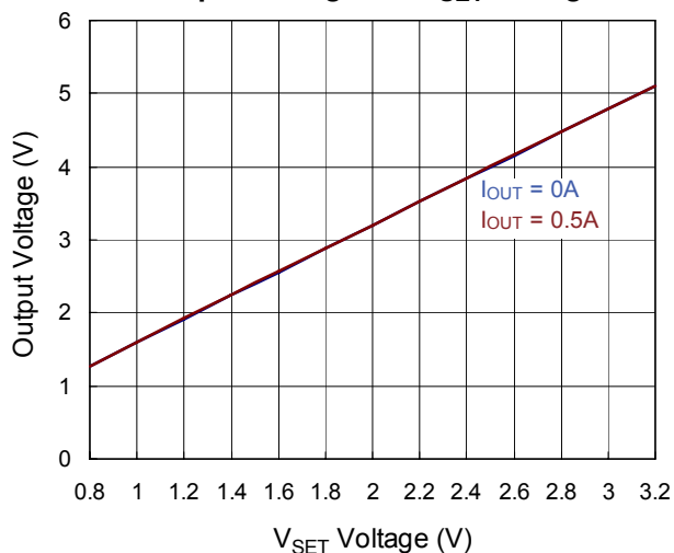
Output Voltage vs. V_{SET} Voltage
