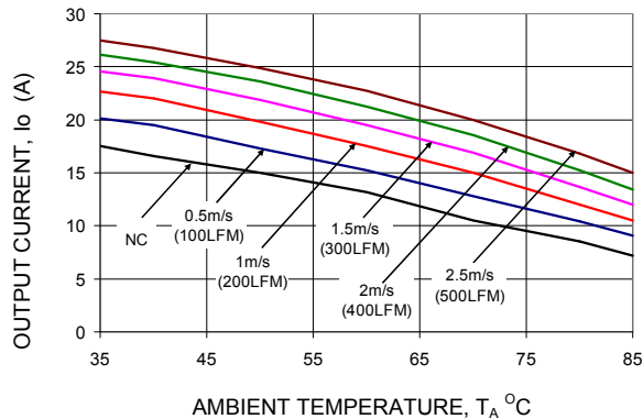
Figure 18. Derating Output Current versus Ambient Temperature and Airflow (ATS030A0X3-SR).
