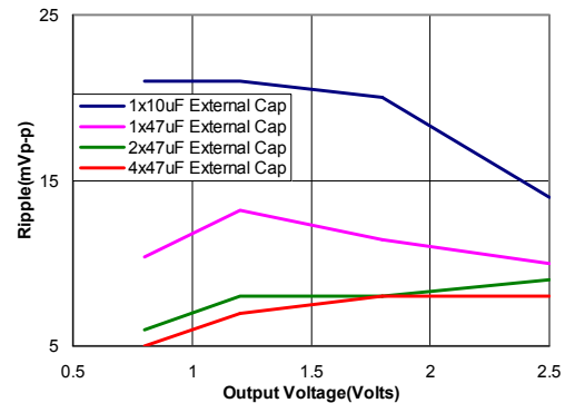
Figure 49. Output ripple voltage for various output voltages with external 1x10 \mu F, 1x47 \mu F, 2x47 \mu F or 4x47 \mu F ceramic capacitors at the output (30A load). Input voltage is 5V.
