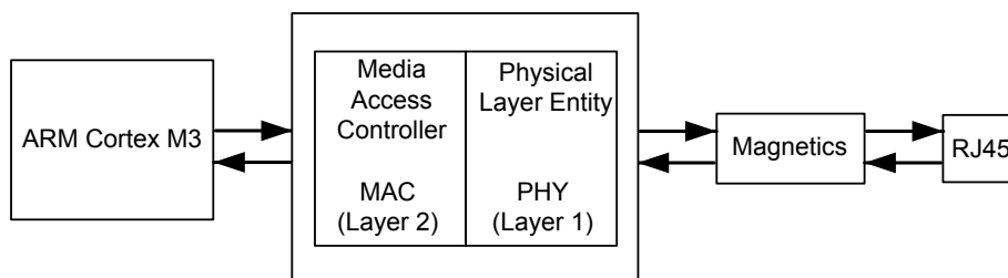
Figure 19-1. Ethernet Controller
