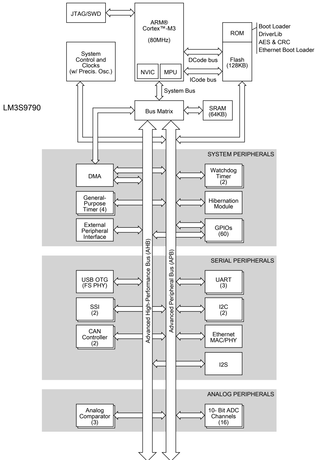
Figure 1-1. Stellaris LM3S9790 Microcontroller High-Level Block Diagram
