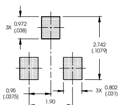
RECOMMENDED FOOTPRINT
