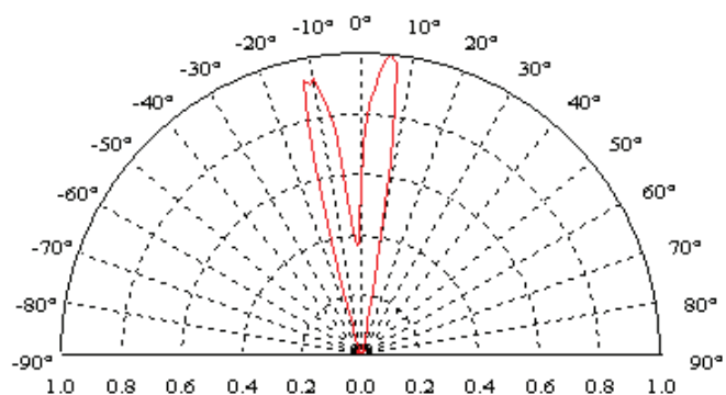
Radiation Pattern
