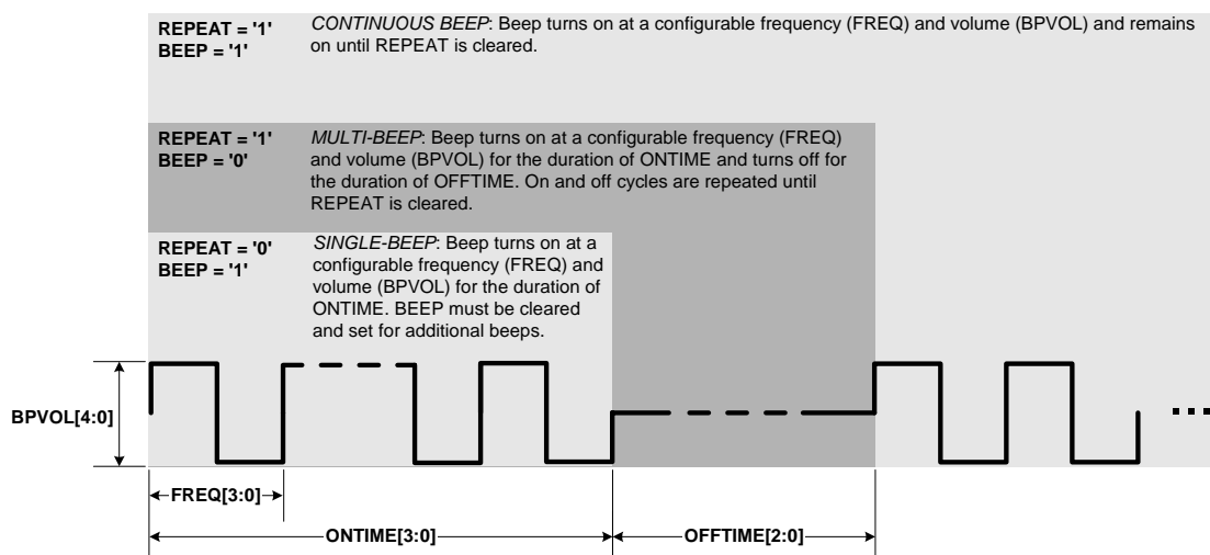
Figure 10. Beep Configuration Options
