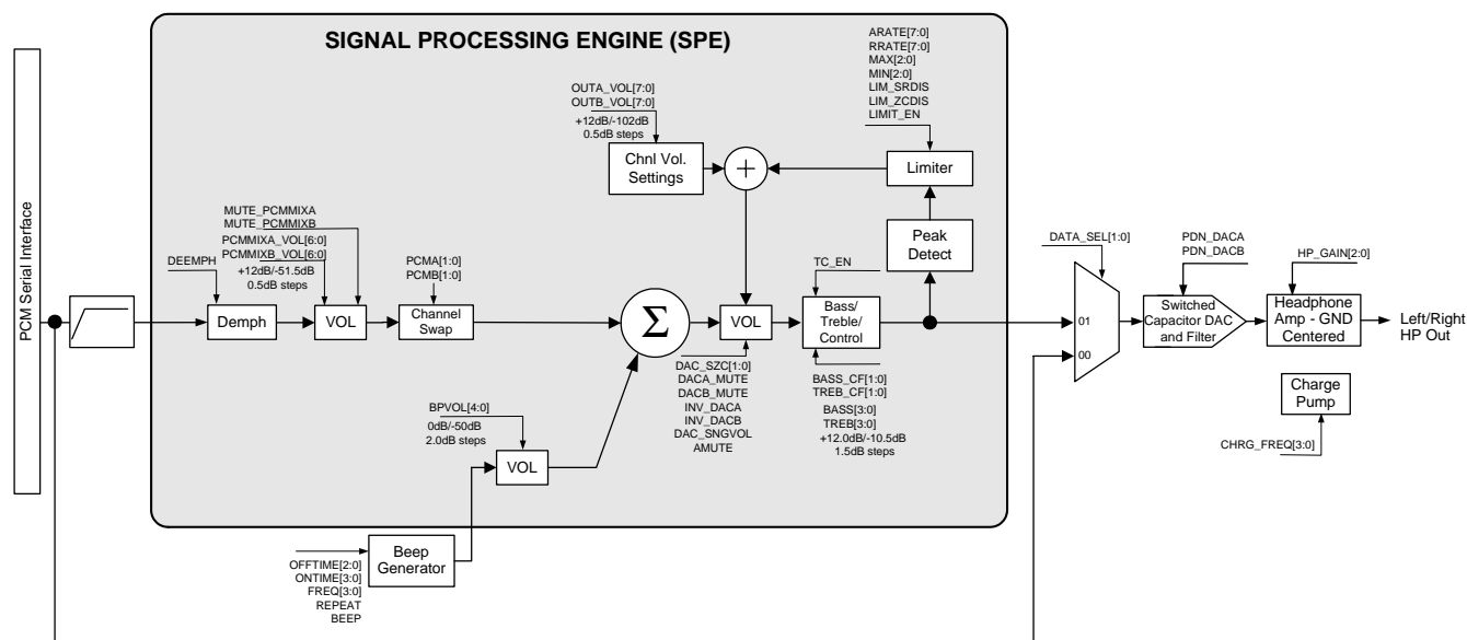
Figure 8. Output Architecture
