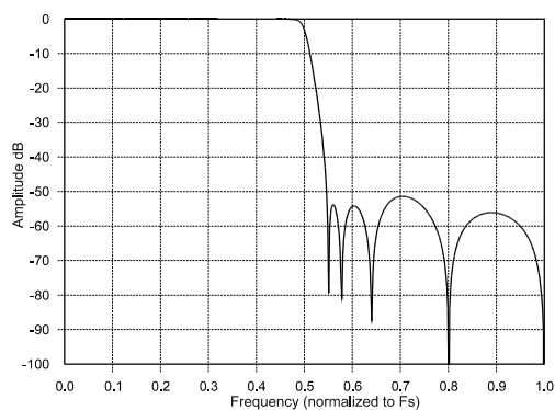
Figure 28. Stopband
