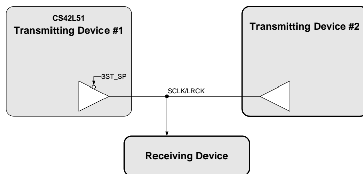
Figure 13. Tri-State SCLK/LRCK
