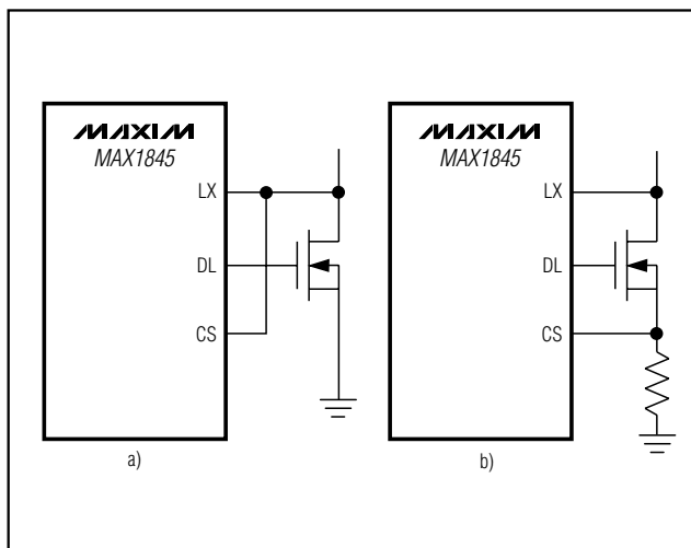
Figure 7. Current-Sense Configurations
