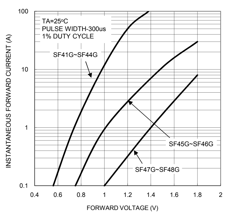
FIG.5- TYPICAL FORWARD CHARACTERISTICS
