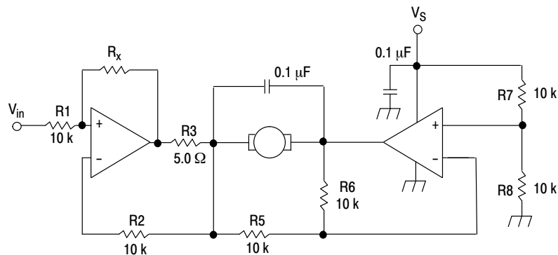
Figure 9. Bidirectional DC Motor Control with Microprocessor-Compatible Inputs
