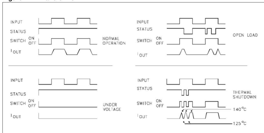
Figure 4. Waveforms
