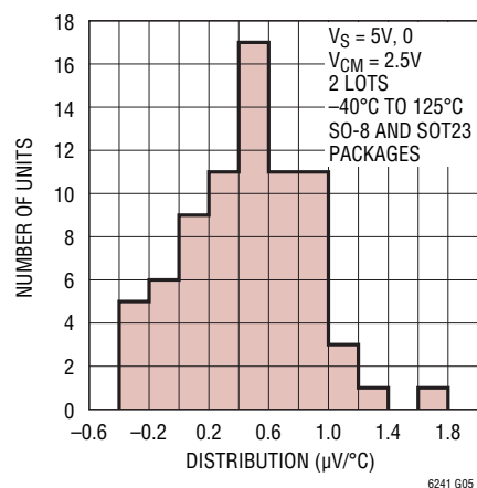
V_{OS} Temperature Coefficient Distribution LTC6240
