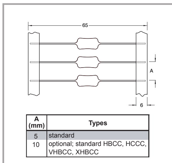
Fig. 5: Radial Taping
