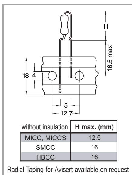
Fig. 5: Radial Taping
