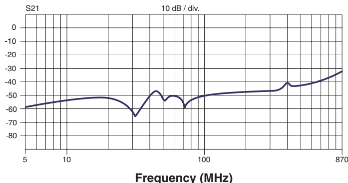
Isolation (TYP)
