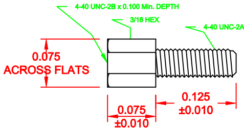
SCREW LOCK
