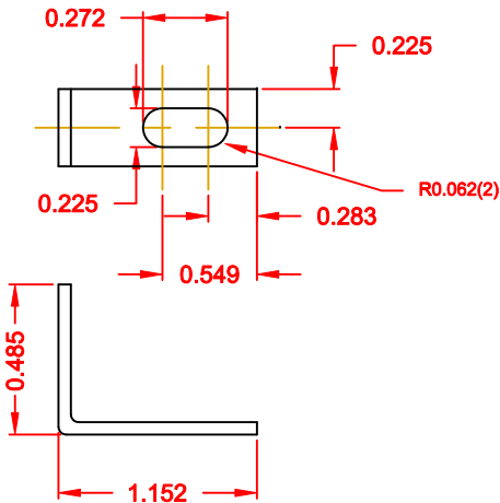
MOUNTING BRACKET
