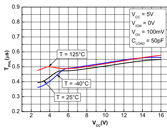
Figure 16. Propagation delay t_{PHL} vs. supply voltage, V_{CC} = 5\text{ V}
