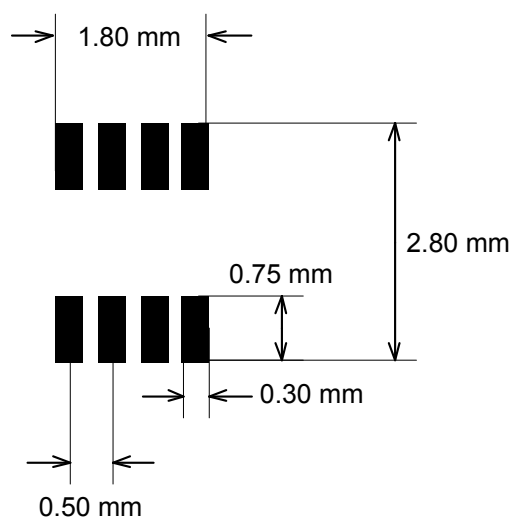
Figure 20. DFN8 2x2 recommended footprint
