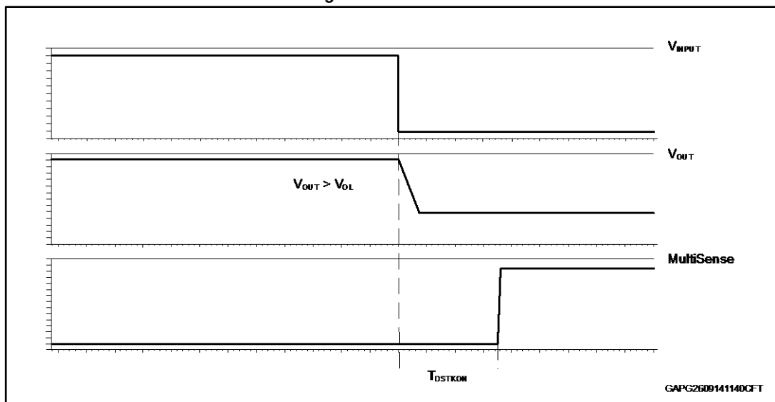
Figure 7: TDSTKON
