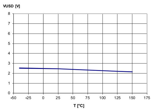
Figure 16: Undervoltage shutdown
