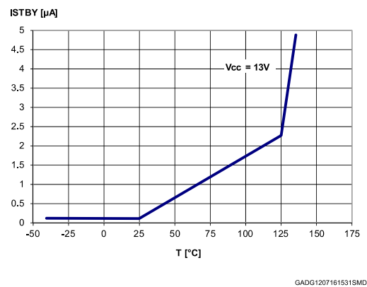
Figure 9: Standby current
