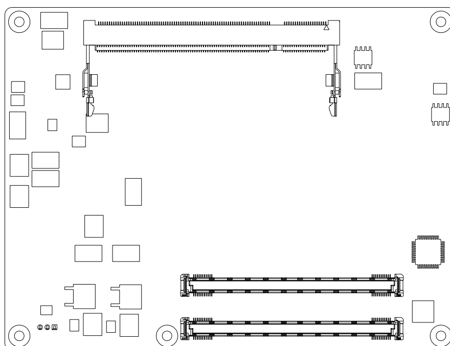
Figure 2.2 Board Layout (rear side)
