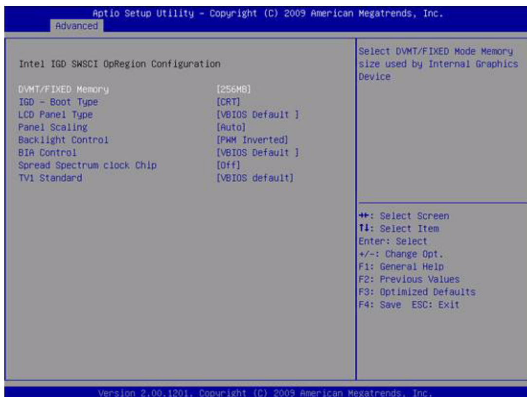
Figure 3.8 IGD Configuration
