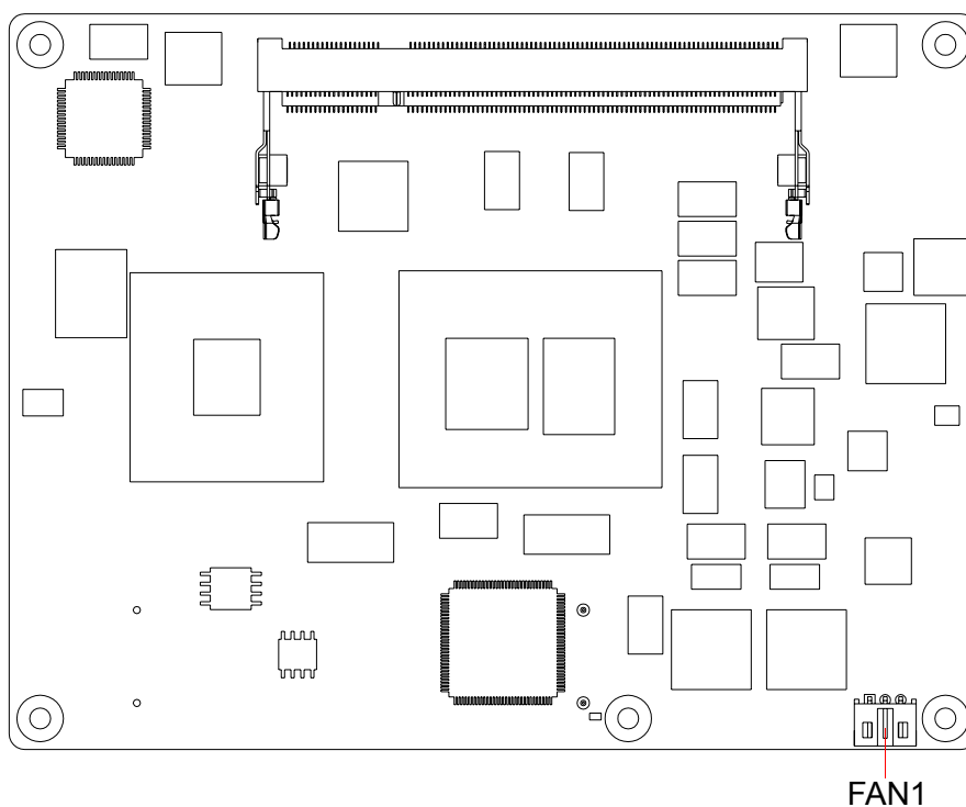
Figure 2.1 Board Layout (front side)
