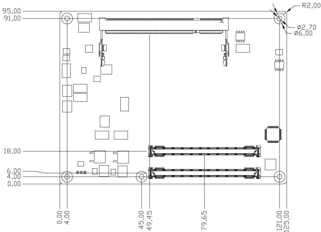
Figure 2.4 Board Dimension (rear side)
