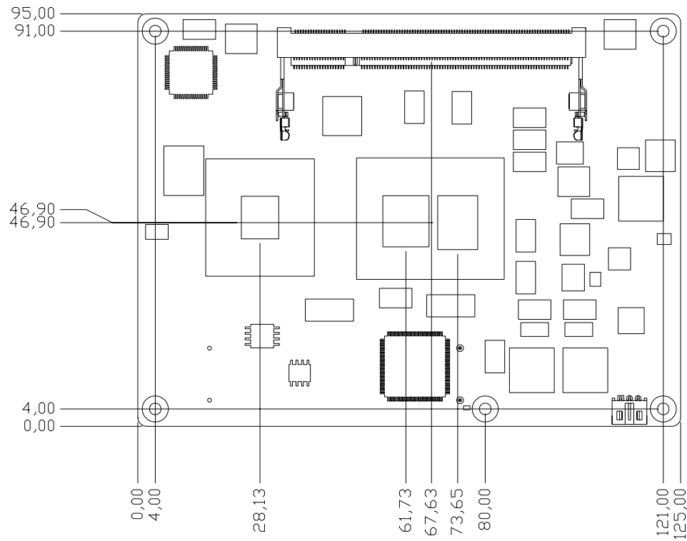
Figure 2.3 Board Dimension (front side)
