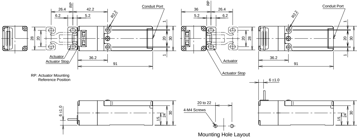
HS5B - using the straight key (HS9Z-A51)
