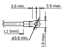
Crimping Terminal 1
