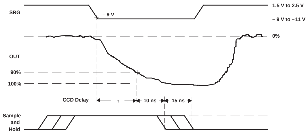
Figure 13. SRG and OUT Waveforms
