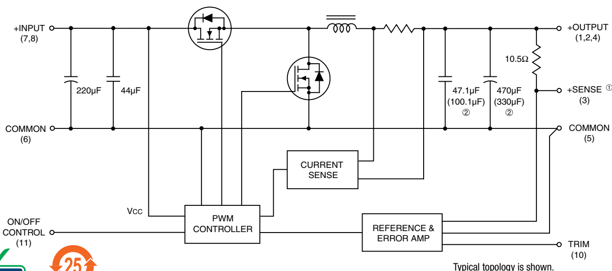
Figure 1. Simplified Schematic
