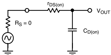
Figure 5. Simplified Model of One Multiplexer Channel
