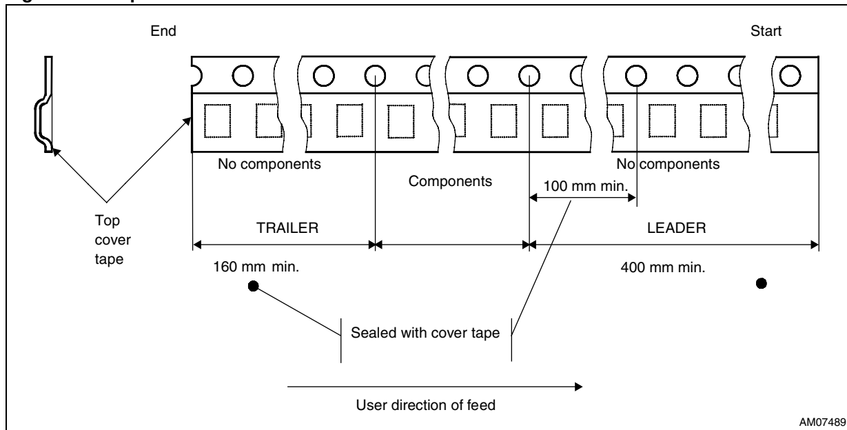
Figure 37. Tape trailer/leader
