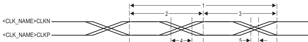
Figure 7-20 Main PLL Transition Time
