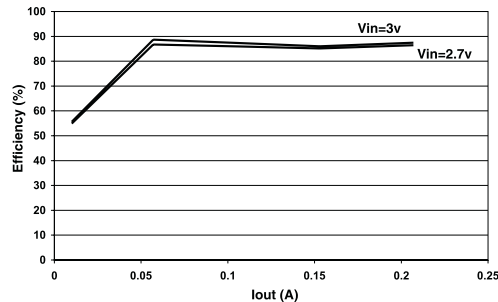
Efficiency vs. Iout *
