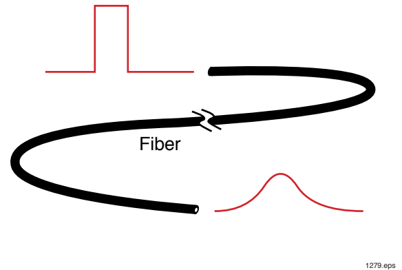
Figure 8. Dispersion in an optical fiber.
