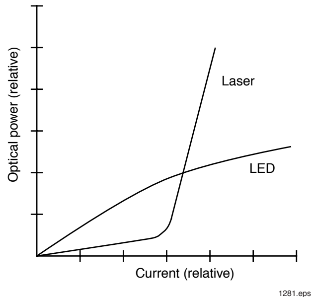
Figure 12. Output optical power versus current for LEDs and laser diodes.
