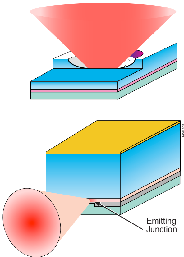
Figure 11. (a) Surface-emitting LED. (b) Edge-emitting LED.
