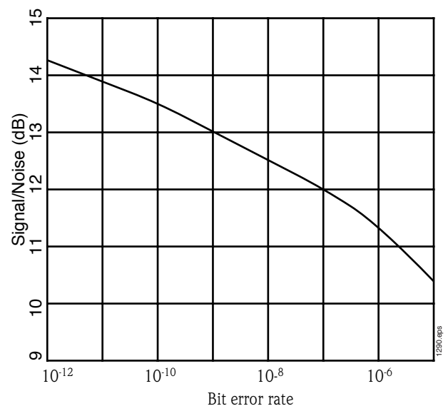
Figure 24. BER versus signal-to-noise ratio.
