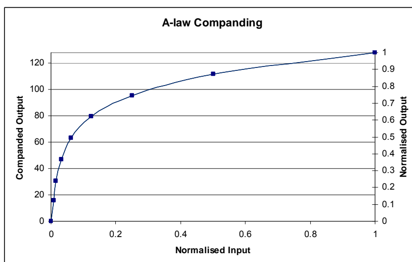
Figure 47 A-Law Companding
