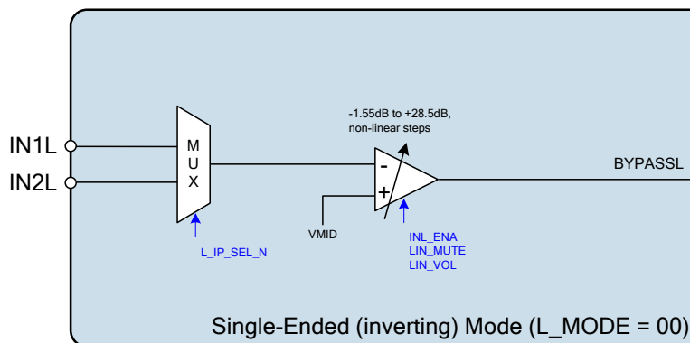
Figure 18 Single Ended Mode
