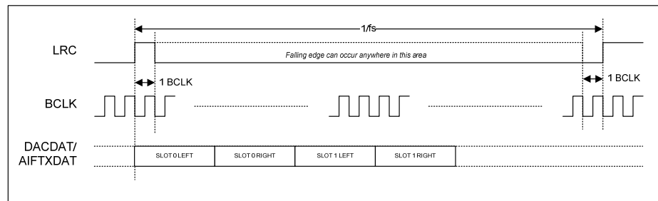
Figure 45 TDM in DSP Mode B
