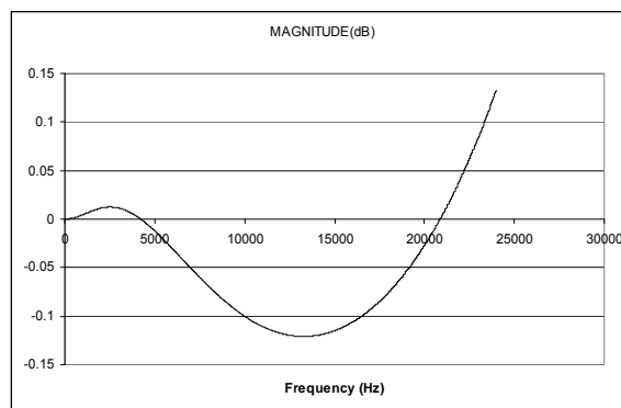
Figure 16 De-Emphasis Error (48kHz)
