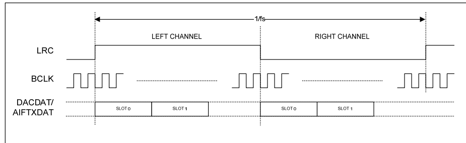
Figure 42 TDM in Left-Justified Mode
