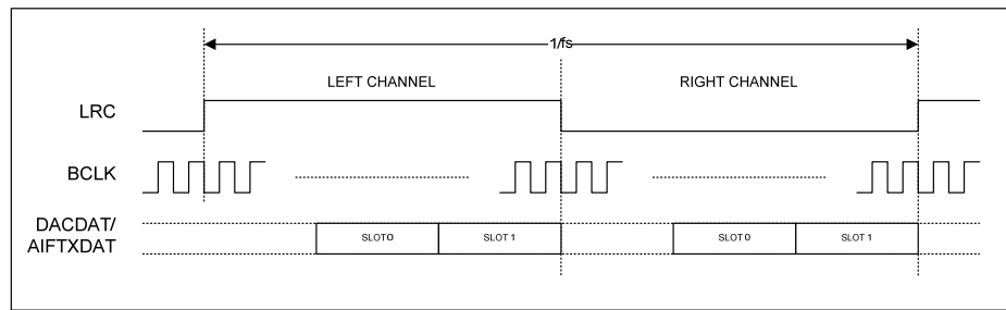
Figure 41 TDM in Right-Justified Mode
