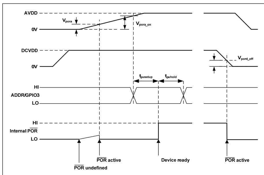
Figure 59 Power On Reset Timing - DCVDD enabled first
