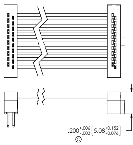
FIG 6 (FFMD-10-T-XX.XX-01-X-N SHOWN) (SAME AS FIG 1, DIFFERENT AS SHOWN)
