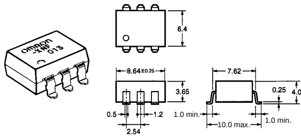
G3VM-XNF G3VM-4NF
